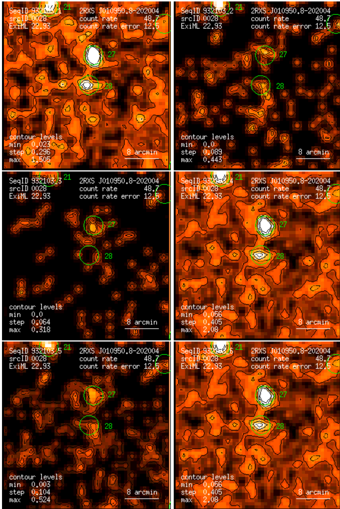
Figure 28: RASS 932103: detection 0028: band rate images, Gaussian filter: (1) PSPC channels 11 – 41, (2) 52 – 90, (3) 91 – 201, (4) 11 – 235, (5) 52 – 201, (6) 11 – 201. Broad band rates in counts/ks. Band rate contour levels in counts/ks/arcmin 2 .
