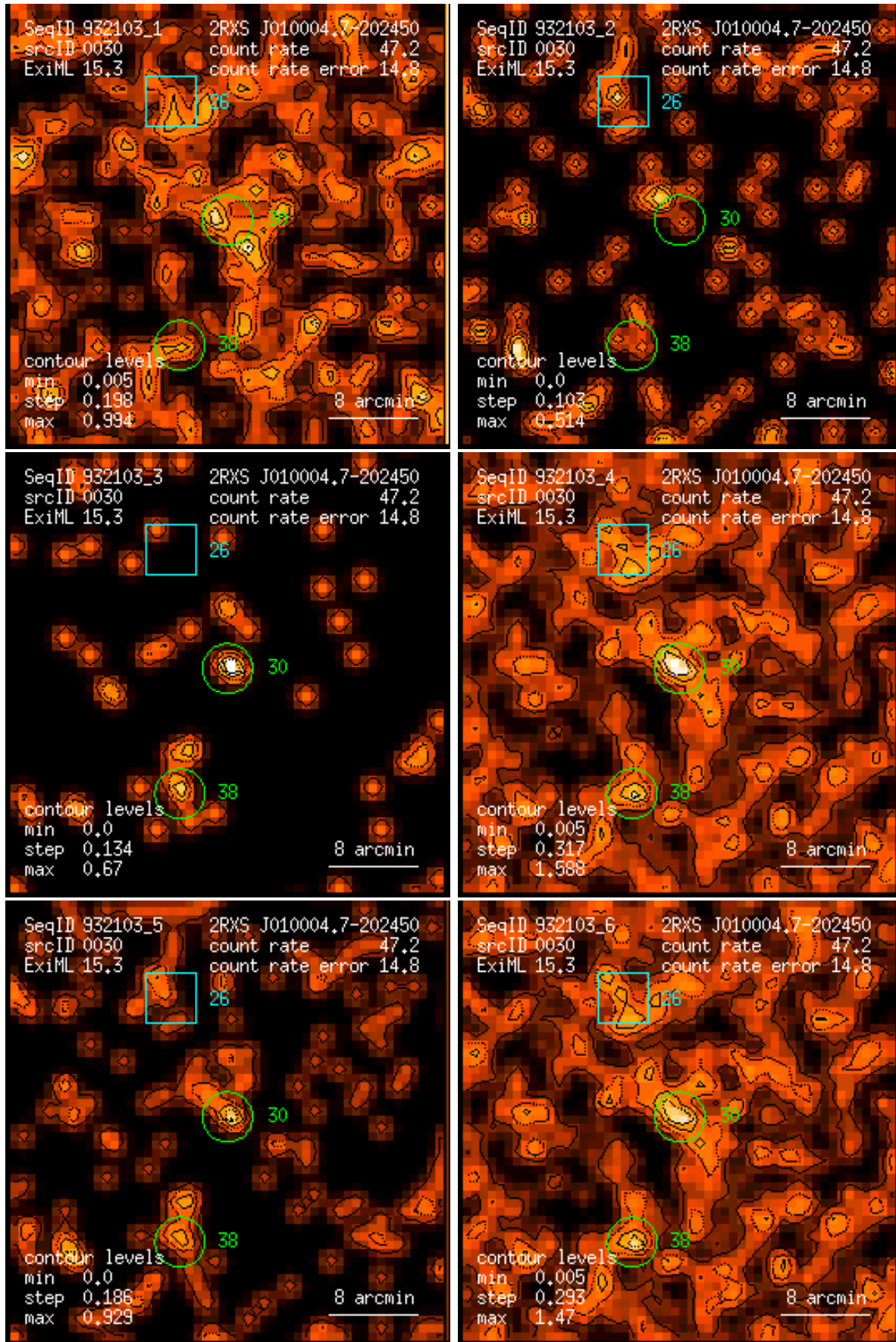
Figure 30: RASS 932103: detection 0030: band rate images, Gaussian filter: (1) PSPC channels 11 – 41, (2) 52 – 90, (3) 91 – 201, (4) 11 – 235, (5) 52 – 201, (6) 11 – 201. Broad band rates in counts/ks. Band rate contour levels in counts/ks/arcmin 2 .
