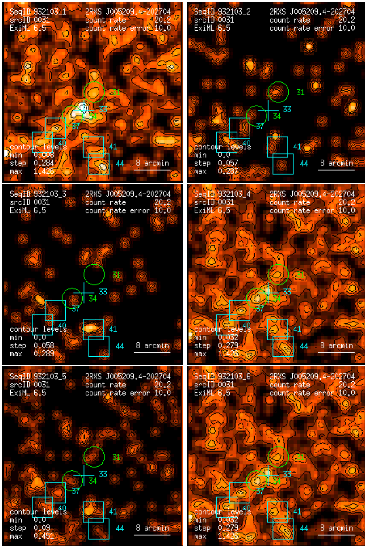
Figure 31: RASS 932103: detection 0031: band rate images, Gaussian filter: (1) PSPC channels 11 – 41, (2) 52 – 90, (3) 91 – 201, (4) 11 – 235, (5) 52 – 201, (6) 11 – 201. Broad band rates in counts/ks. Band rate contour levels in counts/ks/arcmin 2 .
