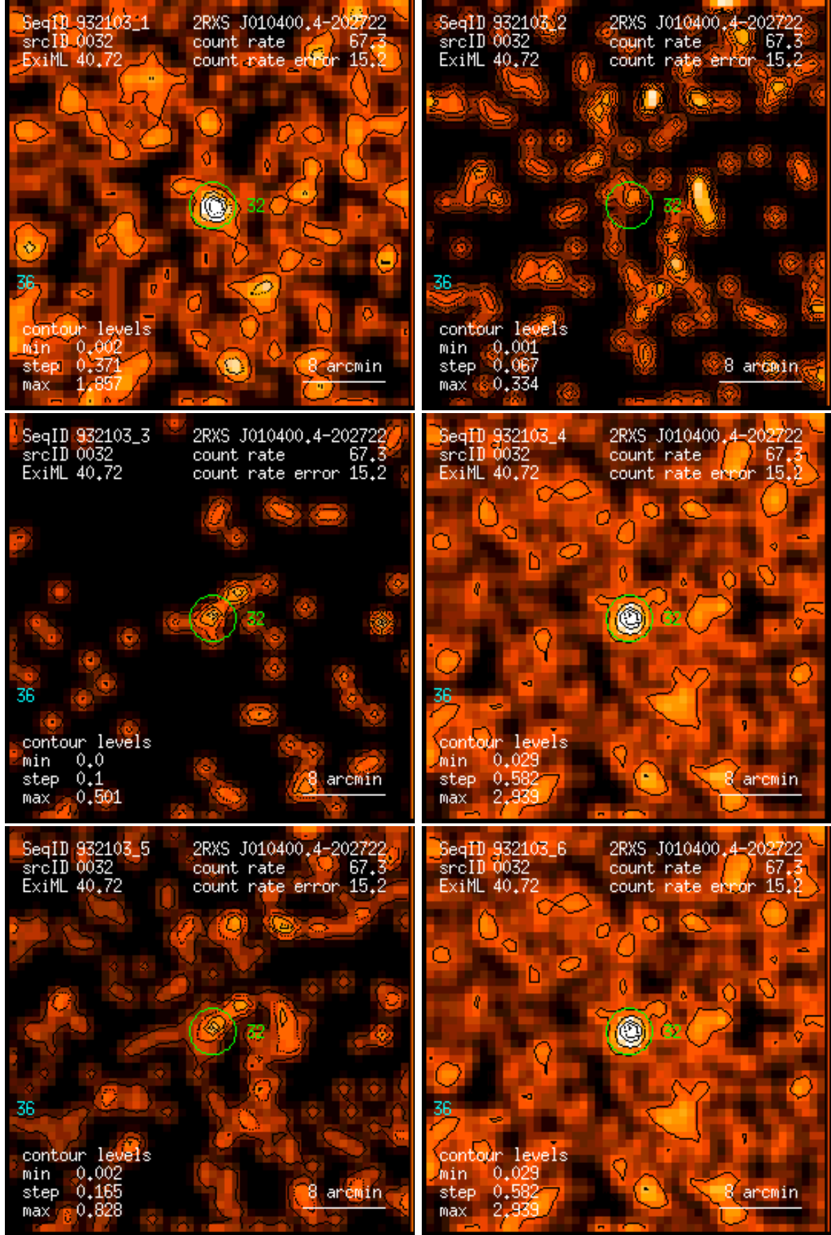
Figure 32: RASS 932103: detection 0032: band rate images, Gaussian filter: (1) PSPC channels 11 – 41, (2) 52 – 90, (3) 91 – 201, (4) 11 – 235, (5) 52 – 201, (6) 11 – 201. Broad band rates in counts/ks. Band rate contour levels in counts/ks/arcmin 2 .
