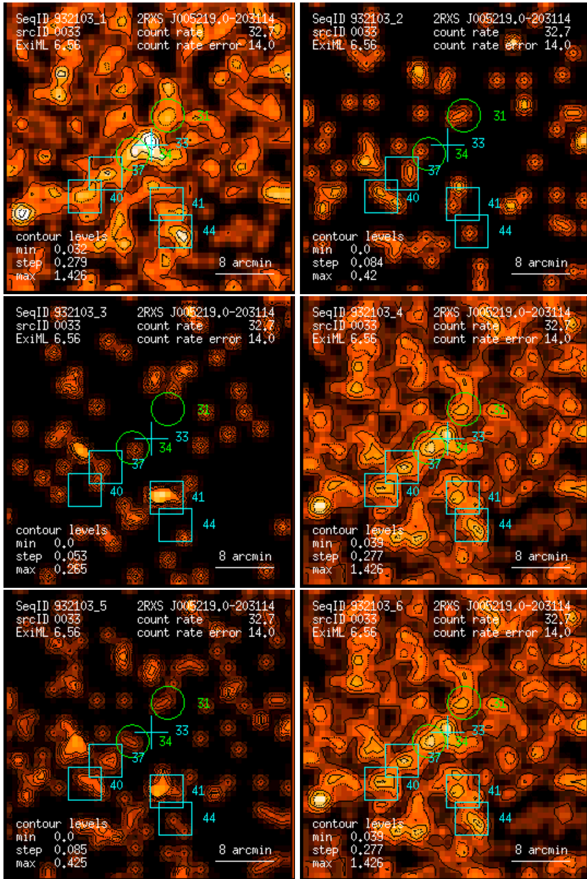
Figure 33: RASS 932103: detection 0033: band rate images, Gaussian filter: (1) PSPC channels 11 – 41, (2) 52 – 90, (3) 91 – 201, (4) 11 – 235, (5) 52 – 201, (6) 11 – 201. Broad band rates in counts/ks. Band rate contour levels in counts/ks/arcmin 2 .
