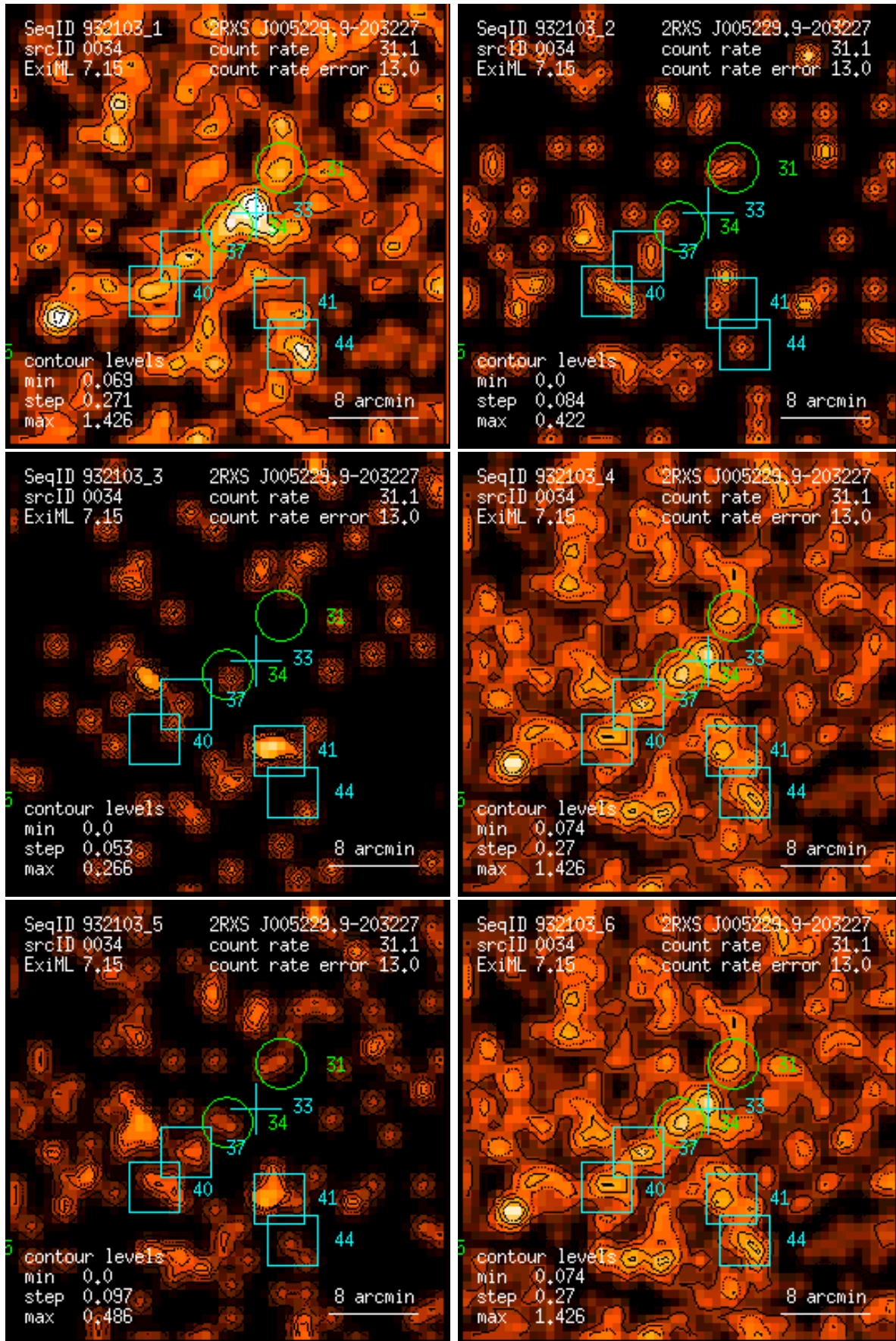
Figure 34: RASS 932103: detection 0034: band rate images, Gaussian filter: (1) PSPC channels 11 – 41, (2) 52 – 90, (3) 91 – 201, (4) 11 – 235, (5) 52 – 201, (6) 11 – 201. Broad band rates in counts/ks. Band rate contour levels in counts/ks/arcmin 2 .
