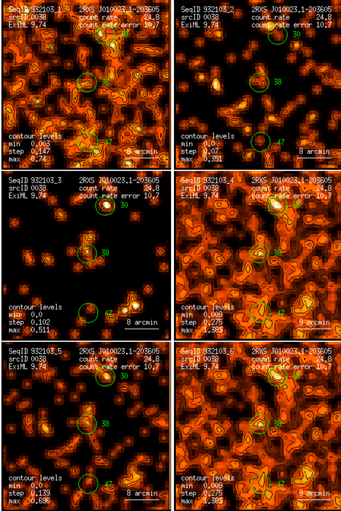
Figure 38: RASS 932103: detection 0038: band rate images, Gaussian filter: (1) PSPC channels 11 – 41, (2) 52 – 90, (3) 91 – 201, (4) 11 – 235, (5) 52 – 201, (6) 11 – 201. Broad band rates in counts/ks. Band rate contour levels in counts/ks/arcmin 2 .
