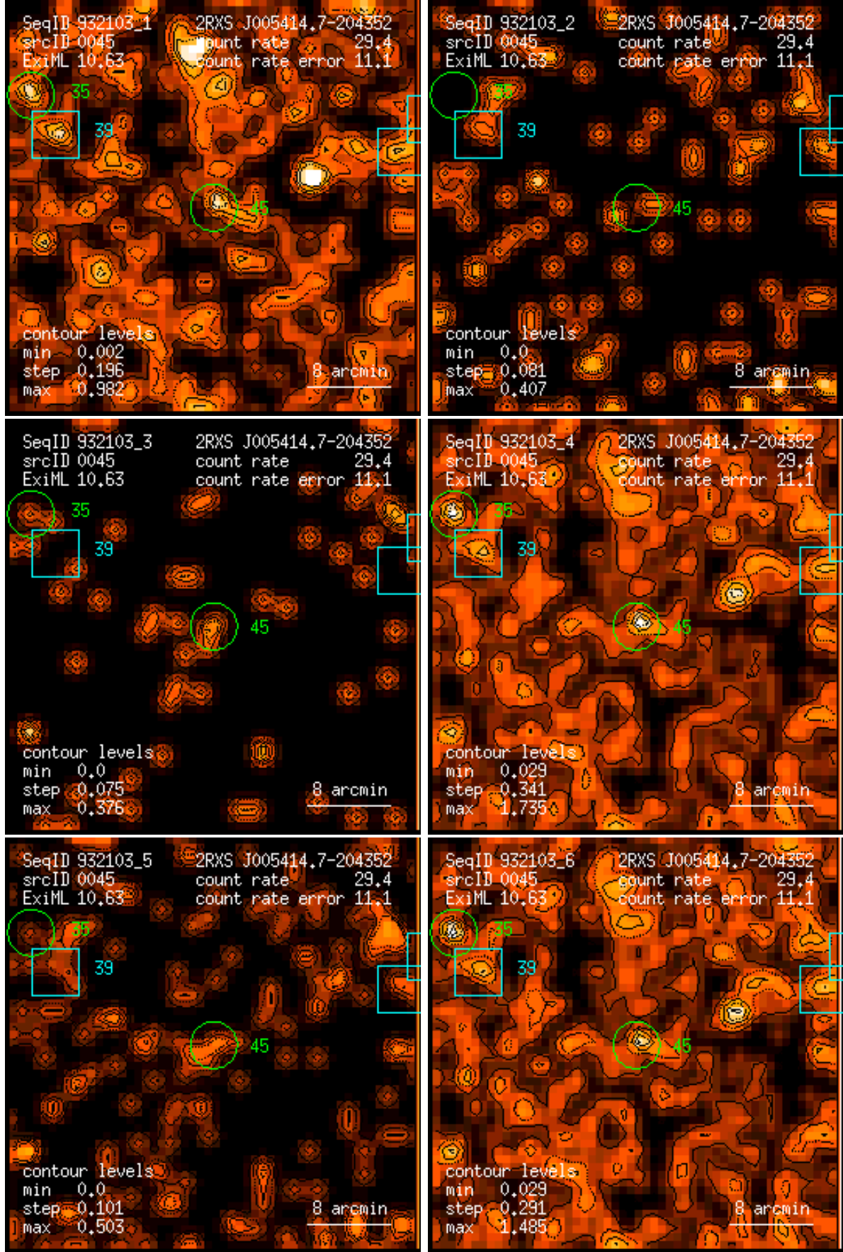
Figure 45: RASS 932103: detection 0045: band rate images, Gaussian filter: (1) PSPC channels 11 – 41, (2) 52 – 90, (3) 91 – 201, (4) 11 – 235, (5) 52 – 201, (6) 11 – 201. Broad band rates in counts/ks. Band rate contour levels in counts/ks/arcmin 2 .
