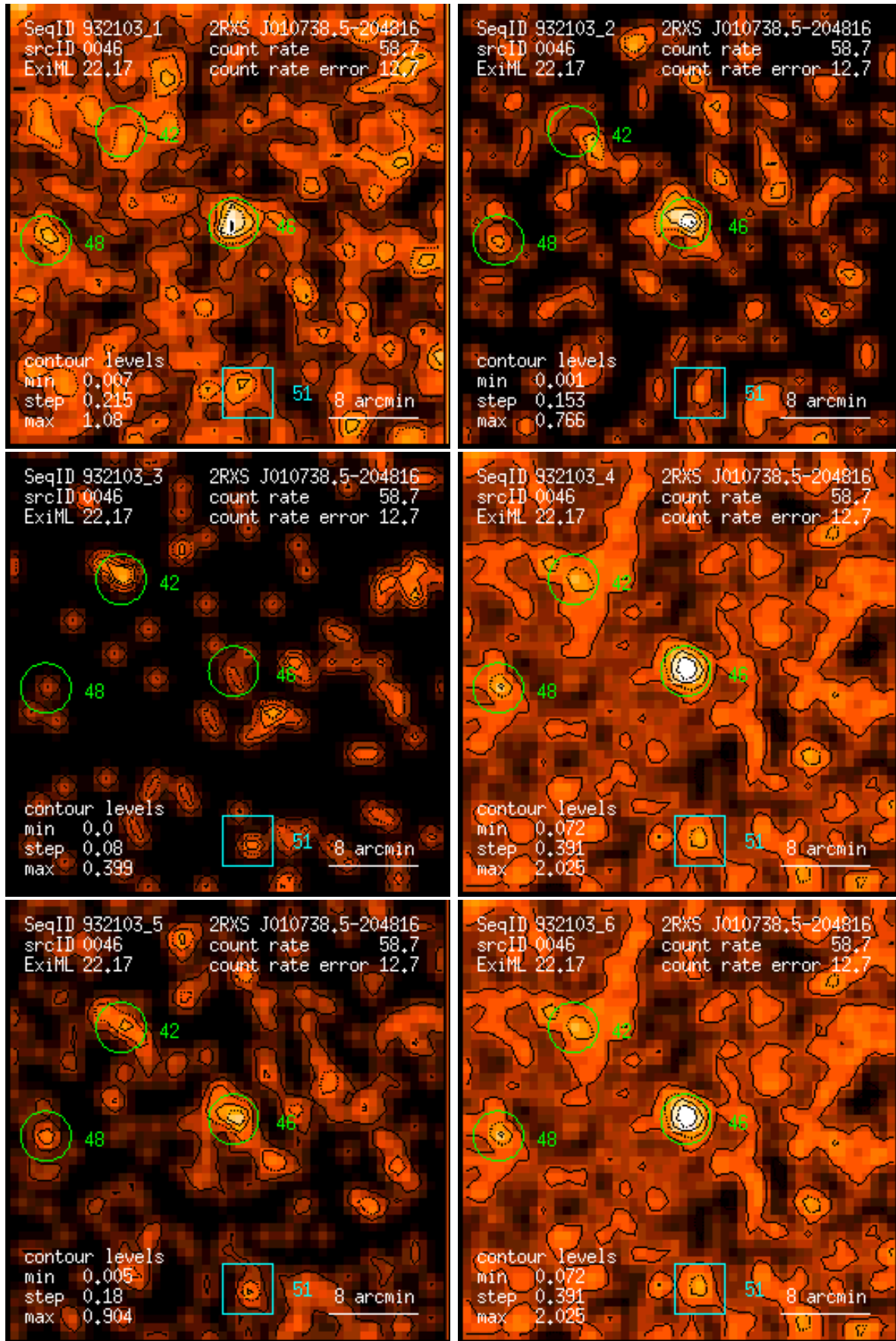
Figure 46: RASS 932103: detection 0046: band rate images, Gaussian filter: (1) PSPC channels 11 – 41, (2) 52 – 90, (3) 91 – 201, (4) 11 – 235, (5) 52 – 201, (6) 11 – 201. Broad band rates in counts/ks. Band rate contour levels in counts/ks/arcmin 2 .
