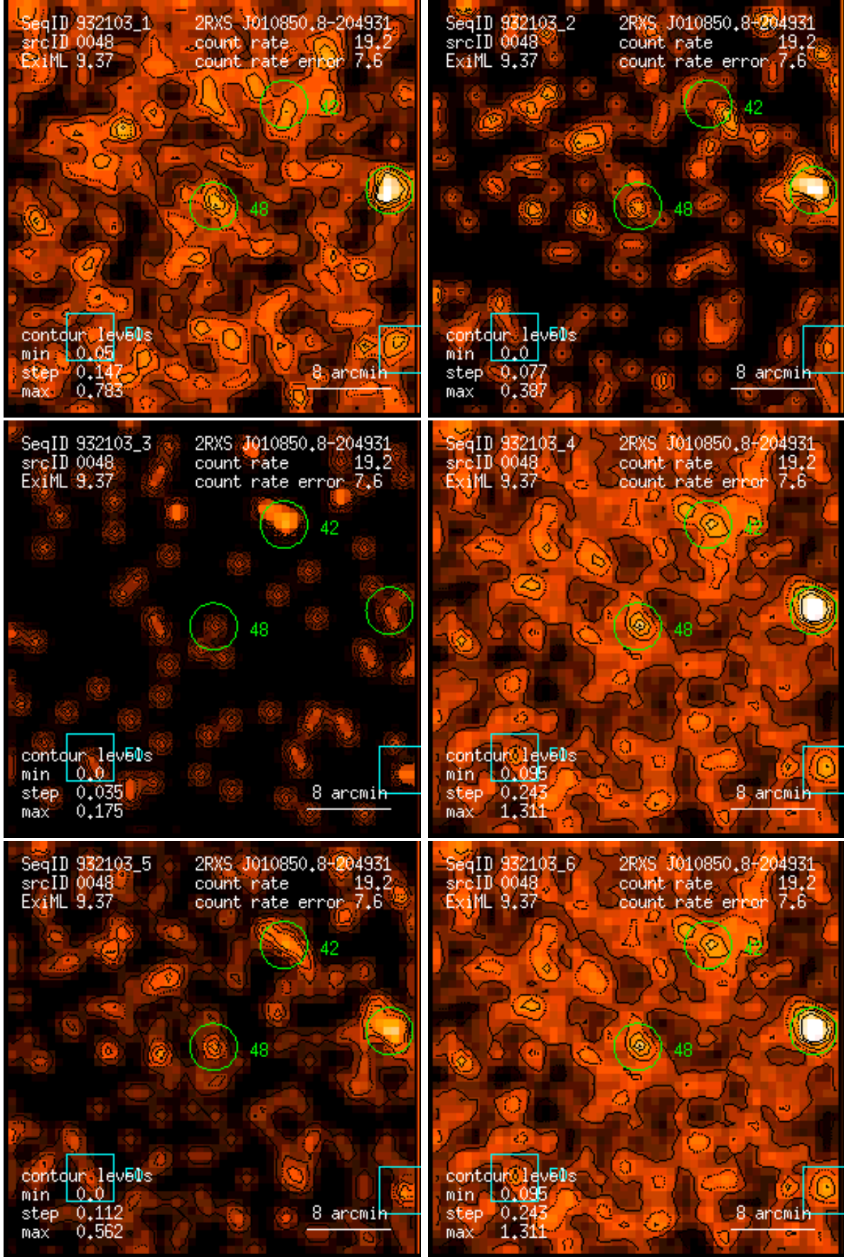
Figure 48: RASS 932103: detection 0048: band rate images, Gaussian filter: (1) PSPC channels 11 – 41, (2) 52 – 90, (3) 91 – 201, (4) 11 – 235, (5) 52 – 201, (6) 11 – 201. Broad band rates in counts/ks. Band rate contour levels in counts/ks/arcmin 2 .
