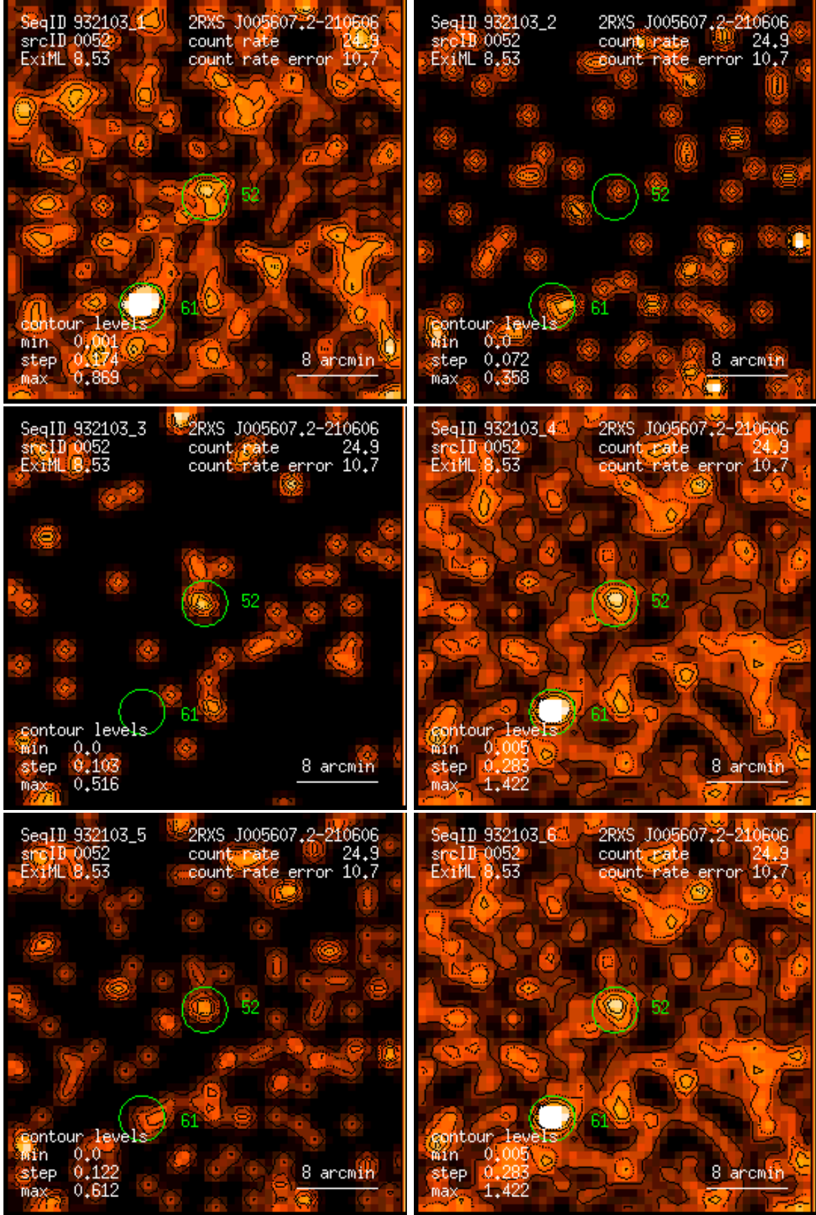
Figure 52: RASS 932103: detection 0052: band rate images, Gaussian filter: (1) PSPC channels 11 – 41, (2) 52 – 90, (3) 91 – 201, (4) 11 – 235, (5) 52 – 201, (6) 11 – 201. Broad band rates in counts/ks. Band rate contour levels in counts/ks/arcmin 2 .
