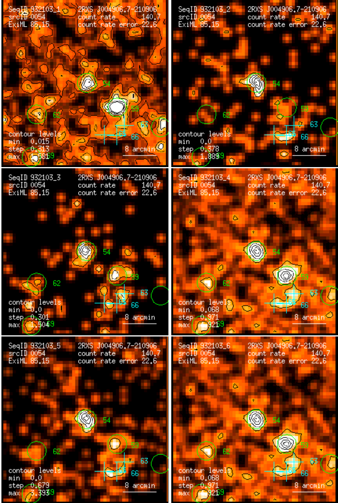
Figure 54: RASS 932103: detection 0054: band rate images, Gaussian filter: (1) PSPC channels 11 – 41, (2) 52 – 90, (3) 91 – 201, (4) 11 – 235, (5) 52 – 201, (6) 11 – 201. Broad band rates in counts/ks. Band rate contour levels in counts/ks/arcmin 2 .
