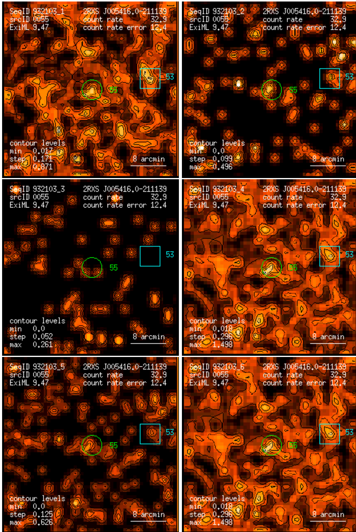
Figure 55: RASS 932103: detection 0055: band rate images, Gaussian filter: (1) PSPC channels 11 – 41, (2) 52 – 90, (3) 91 – 201, (4) 11 – 235, (5) 52 – 201, (6) 11 – 201. Broad band rates in counts/ks. Band rate contour levels in counts/ks/arcmin 2 .
