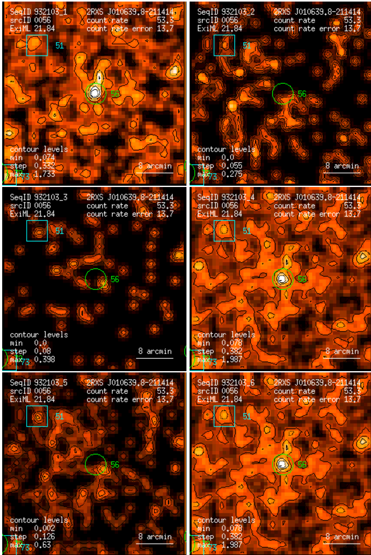
Figure 56: RASS 932103: detection 0056: band rate images, Gaussian filter: (1) PSPC channels 11 – 41, (2) 52 – 90, (3) 91 – 201, (4) 11 – 235, (5) 52 – 201, (6) 11 – 201. Broad band rates in counts/ks. Band rate contour levels in counts/ks/arcmin 2 .
