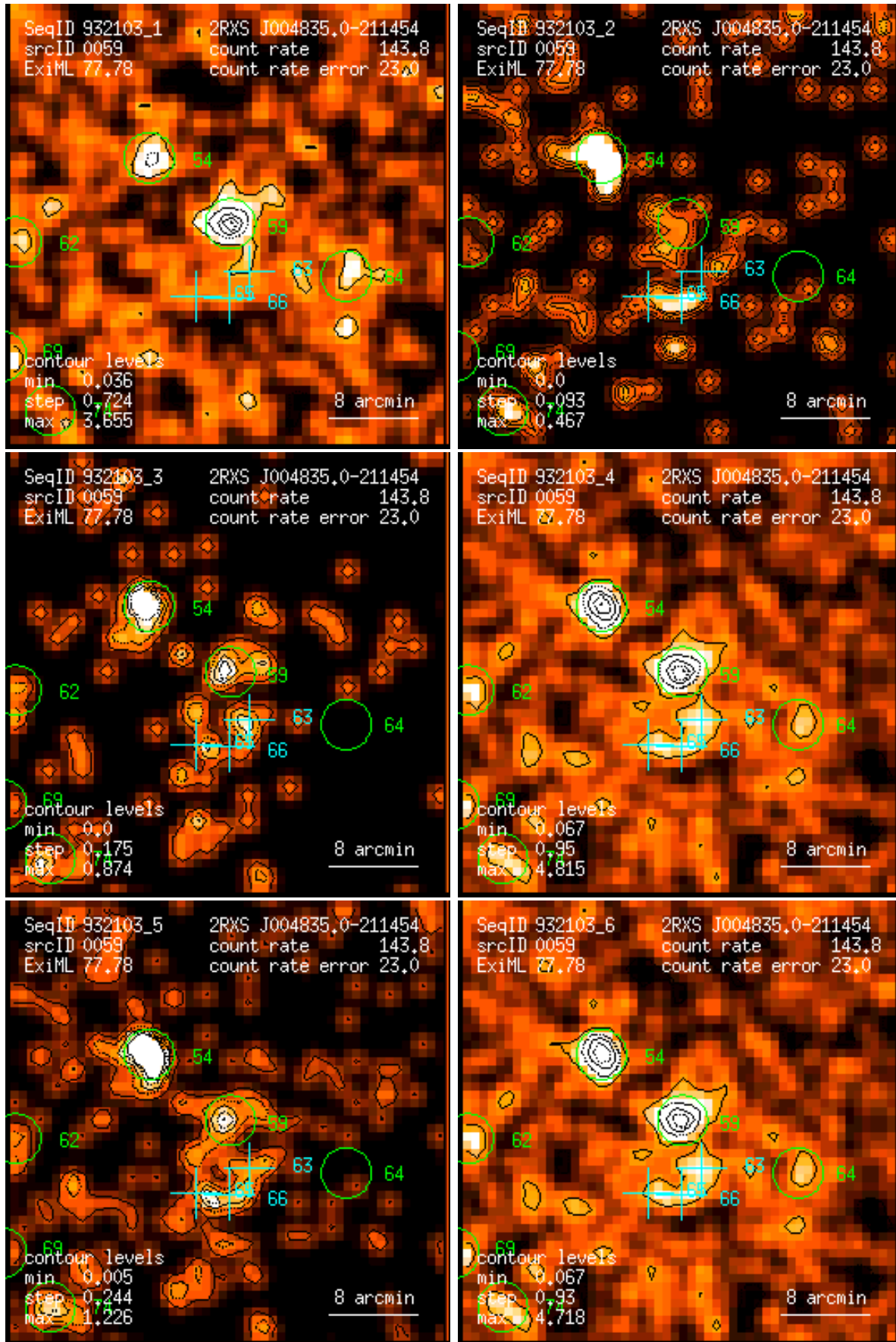
Figure 59: RASS 932103: detection 0059: band rate images, Gaussian filter: (1) PSPC channels 11 – 41, (2) 52 – 90, (3) 91 – 201, (4) 11 – 235, (5) 52 – 201, (6) 11 – 201. Broad band rates in counts/ks. Band rate contour levels in counts/ks/arcmin 2 .
