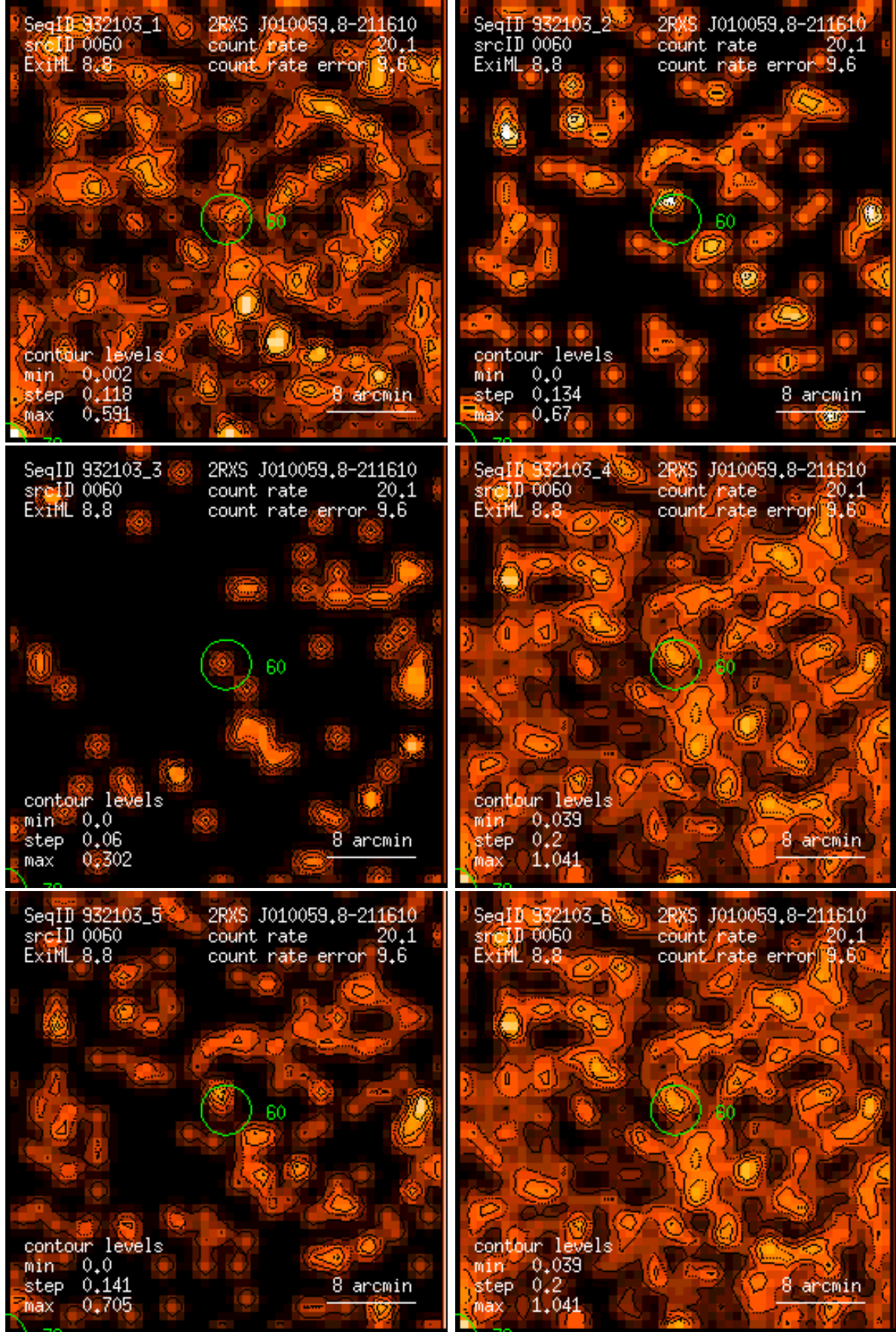
Figure 60: RASS 932103: detection 0060: band rate images, Gaussian filter: (1) PSPC channels 11 – 41, (2) 52 – 90, (3) 91 – 201, (4) 11 – 235, (5) 52 – 201, (6) 11 – 201. Broad band rates in counts/ks. Band rate contour levels in counts/ks/arcmin 2 .
