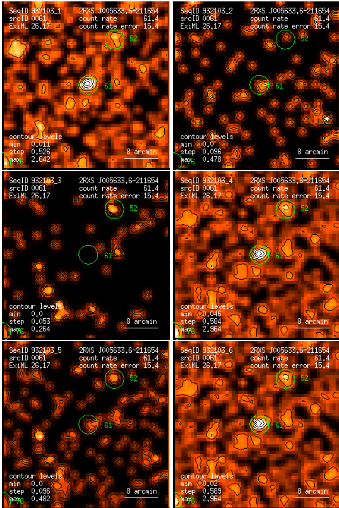
Figure 61: RASS 932103: detection 0061: band rate images, Gaussian filter: (1) PSPC channels 11 – 41, (2) 52 – 90, (3) 91 – 201, (4) 11 – 235, (5) 52 – 201, (6) 11 – 201. Broad band rates in counts/ks. Band rate contour levels in counts/ks/arcmin 2 .
