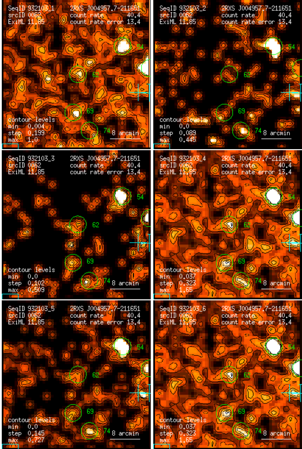
Figure 62: RASS 932103: detection 0062: band rate images, Gaussian filter: (1) PSPC channels 11 – 41, (2) 52 – 90, (3) 91 – 201, (4) 11 – 235, (5) 52 – 201, (6) 11 – 201. Broad band rates in counts/ks. Band rate contour levels in counts/ks/arcmin 2 .
