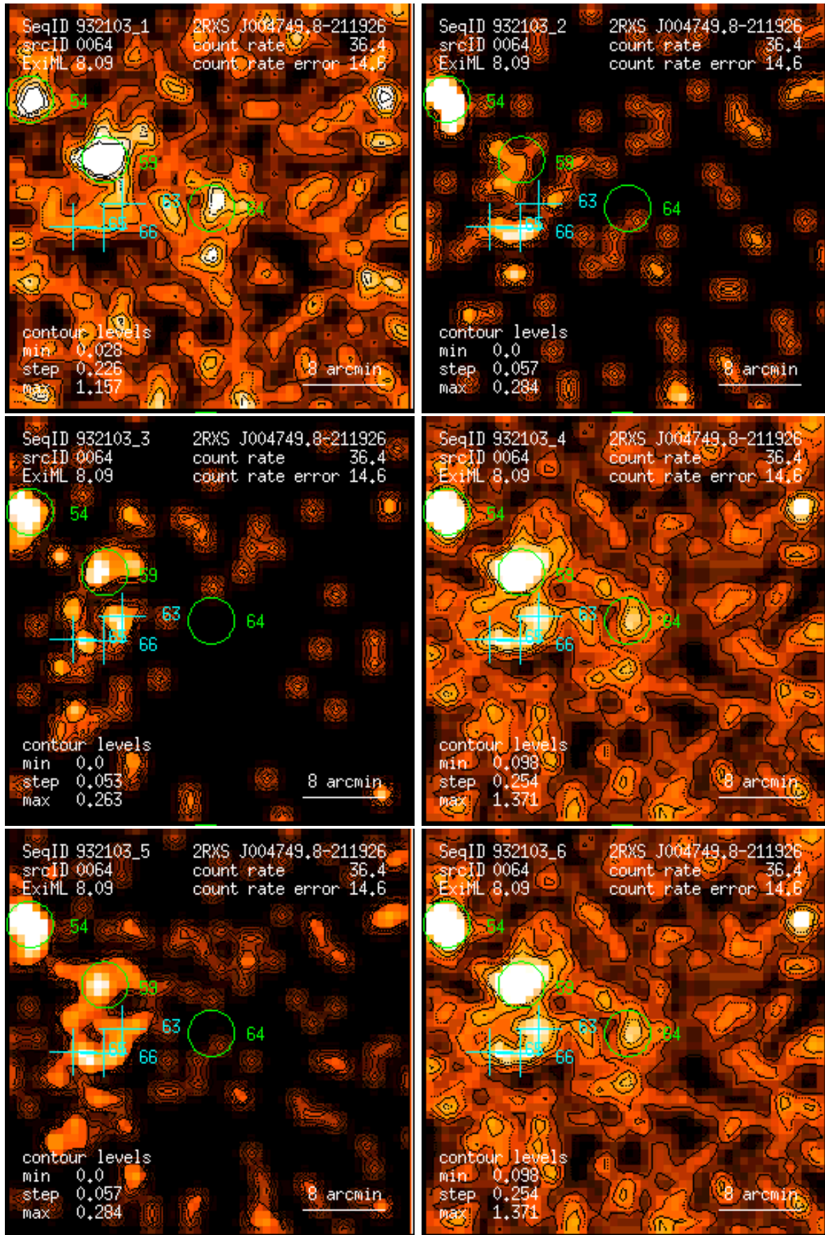
Figure 64: RASS 932103: detection 0064: band rate images, Gaussian filter: (1) PSPC channels 11 – 41, (2) 52 – 90, (3) 91 – 201, (4) 11 – 235, (5) 52 – 201, (6) 11 – 201. Broad band rates in counts/ks. Band rate contour levels in counts/ks/arcmin 2 .
