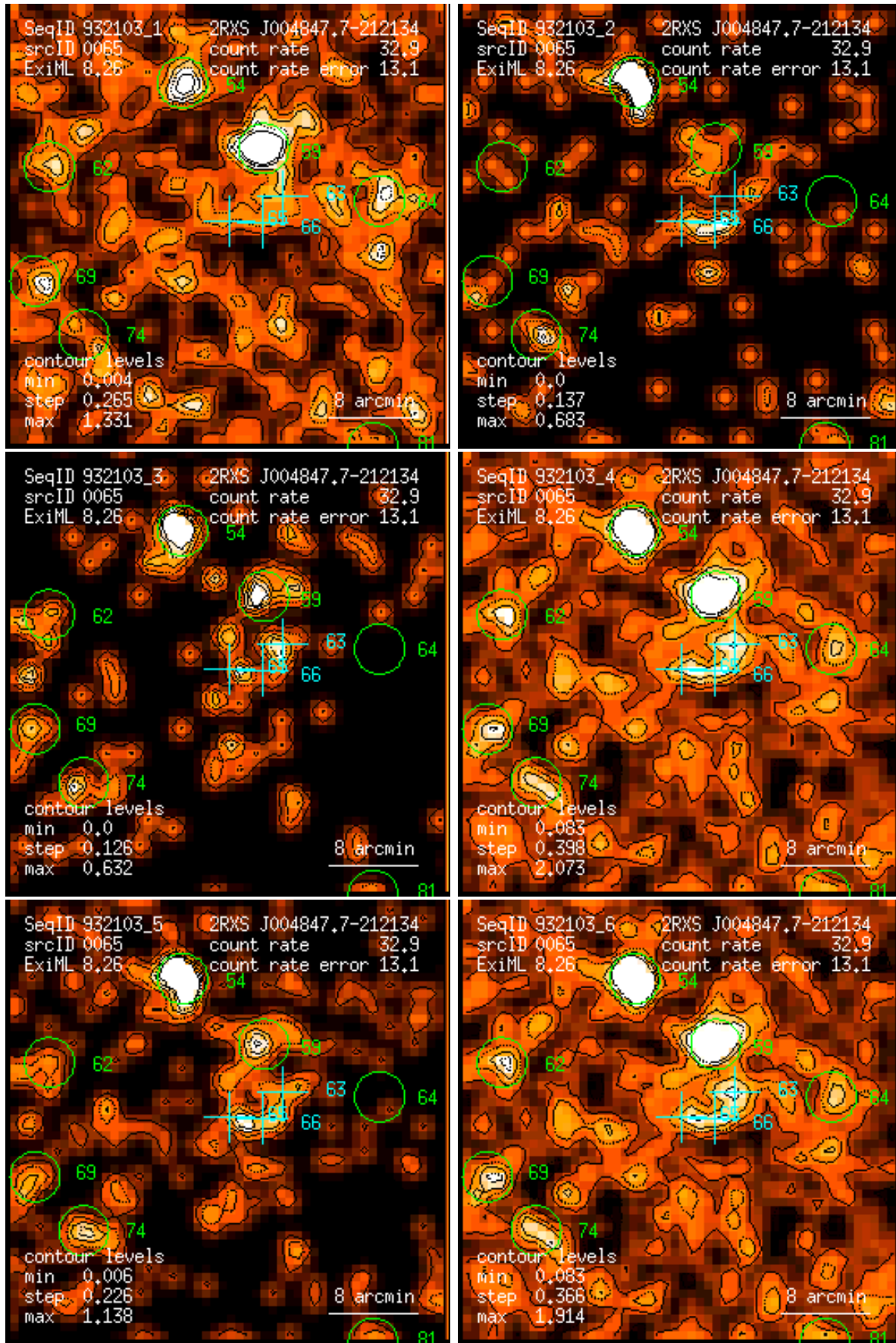
Figure 65: RASS 932103: detection 0065: band rate images, Gaussian filter: (1) PSPC channels 11 – 41, (2) 52 – 90, (3) 91 – 201, (4) 11 – 235, (5) 52 – 201, (6) 11 – 201. Broad band rates in counts/ks. Band rate contour levels in counts/ks/arcmin 2 .
