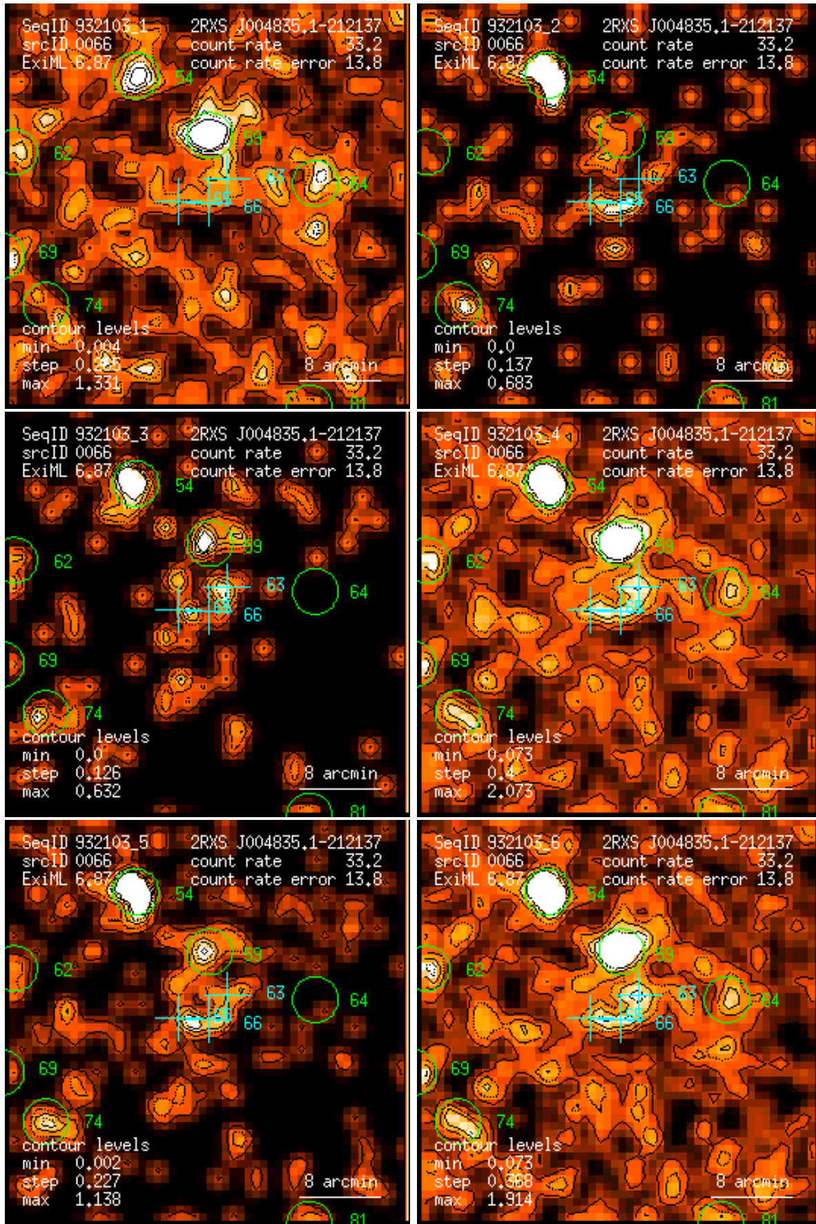
Figure 66: RASS 932103: detection 0066: band rate images, Gaussian filter: (1) PSPC channels 11 – 41, (2) 52 – 90, (3) 91 – 201, (4) 11 – 235, (5) 52 – 201, (6) 11 – 201. Broad band rates in counts/ks. Band rate contour levels in counts/ks/arcmin 2 .
