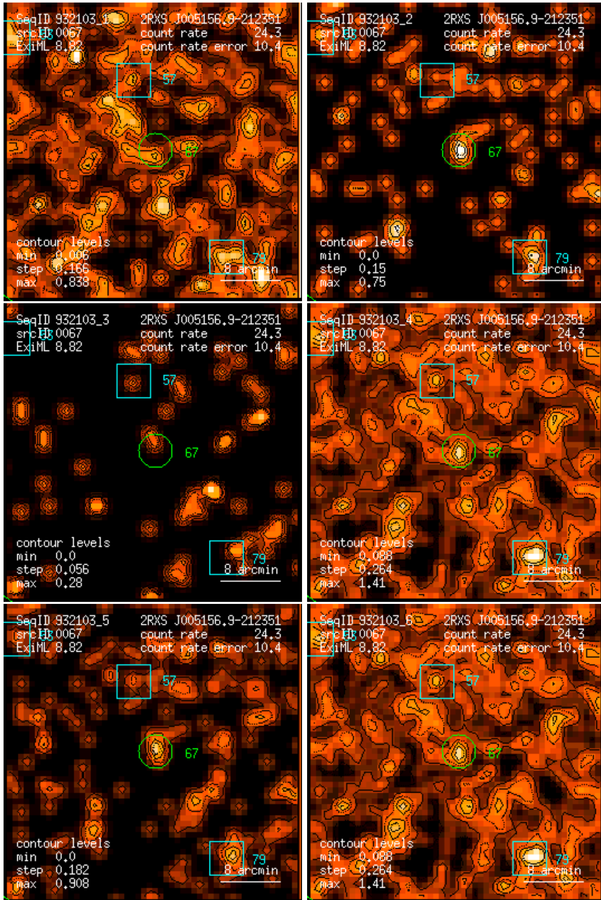
Figure 67: RASS 932103: detection 0067: band rate images, Gaussian filter: (1) PSPC channels 11 – 41, (2) 52 – 90, (3) 91 – 201, (4) 11 – 235, (5) 52 – 201, (6) 11 – 201. Broad band rates in counts/ks. Band rate contour levels in counts/ks/arcmin 2 .
