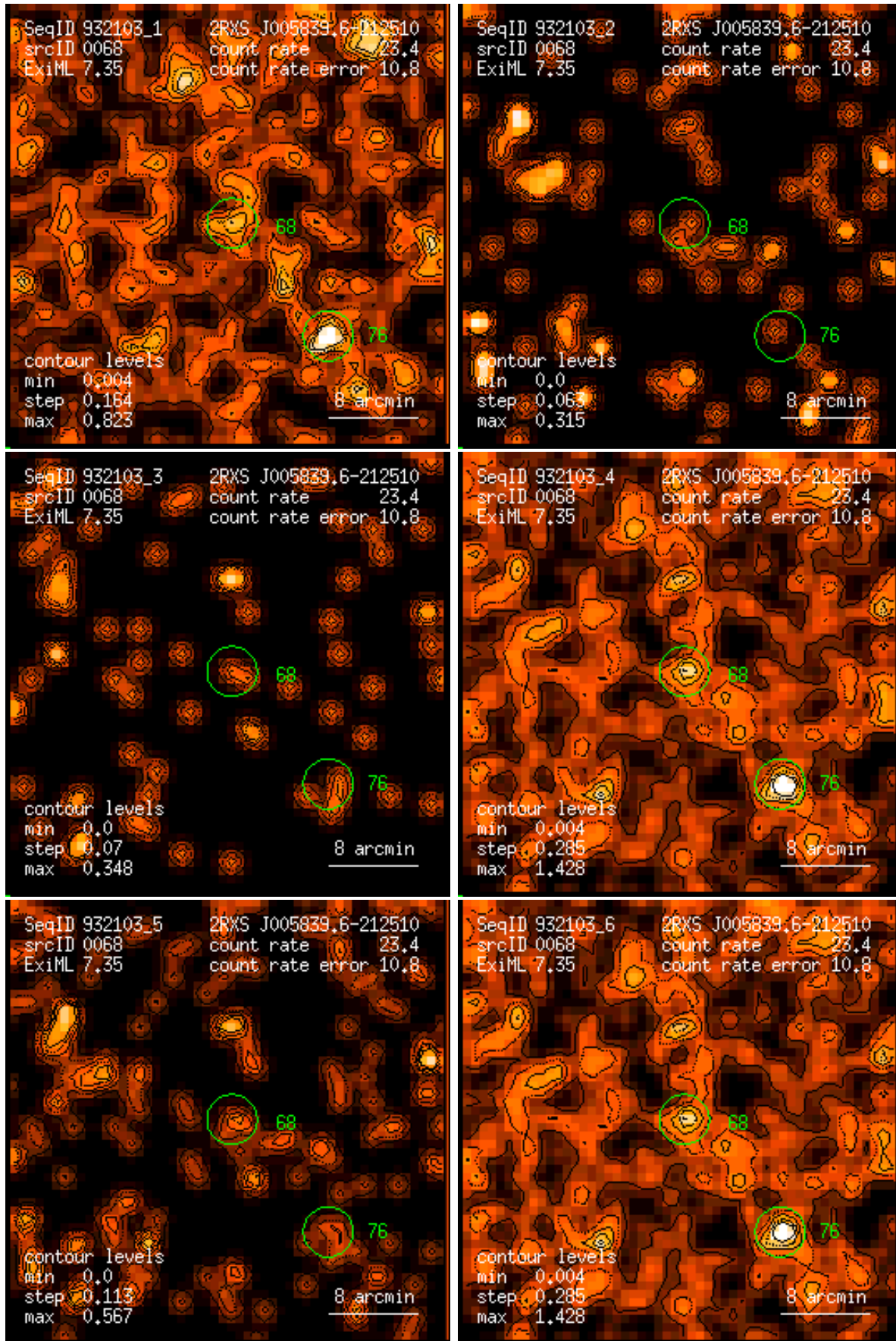
Figure 68: RASS 932103: detection 0068: band rate images, Gaussian filter: (1) PSPC channels 11 – 41, (2) 52 – 90, (3) 91 – 201, (4) 11 – 235, (5) 52 – 201, (6) 11 – 201. Broad band rates in counts/ks. Band rate contour levels in counts/ks/arcmin 2 .
