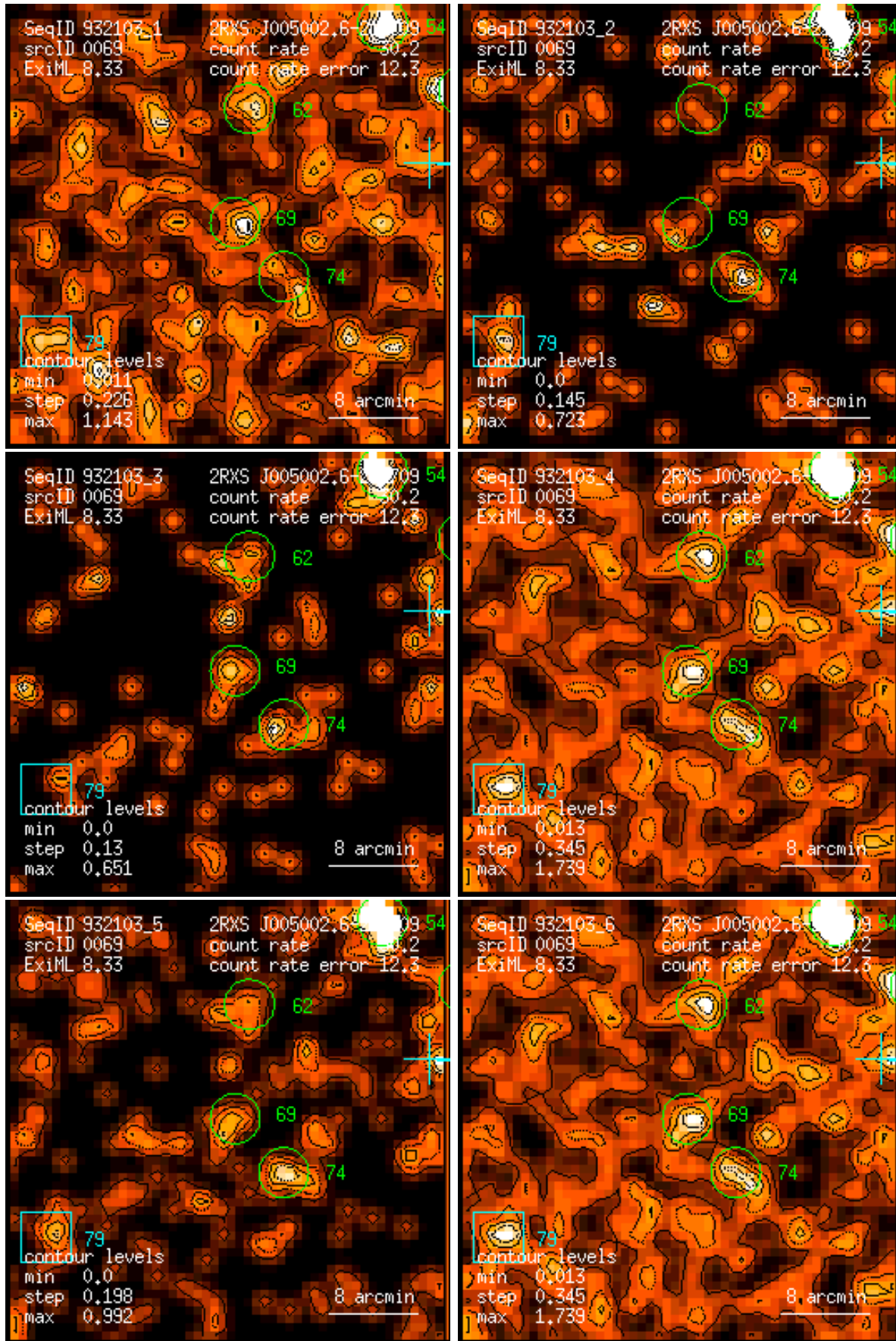
Figure 69: RASS 932103: detection 0069: band rate images, Gaussian filter: (1) PSPC channels 11 – 41, (2) 52 – 90, (3) 91 – 201, (4) 11 – 235, (5) 52 – 201, (6) 11 – 201. Broad band rates in counts/ks. Band rate contour levels in counts/ks/arcmin 2 .
