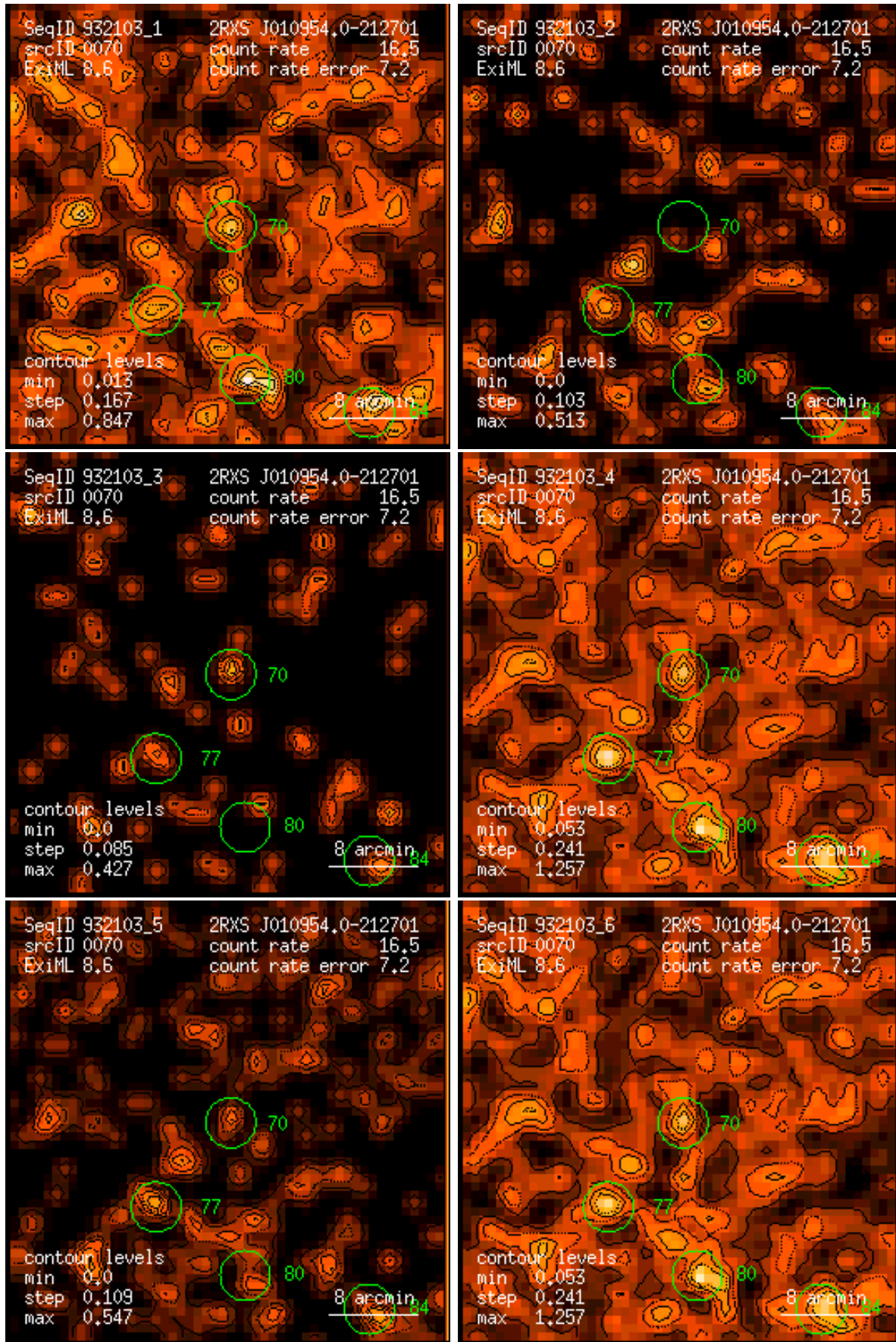
Figure 70: RASS 932103: detection 0070: band rate images, Gaussian filter: (1) PSPC channels 11 – 41, (2) 52 – 90, (3) 91 – 201, (4) 11 – 235, (5) 52 – 201, (6) 11 – 201. Broad band rates in counts/ks. Band rate contour levels in counts/ks/arcmin 2 .
