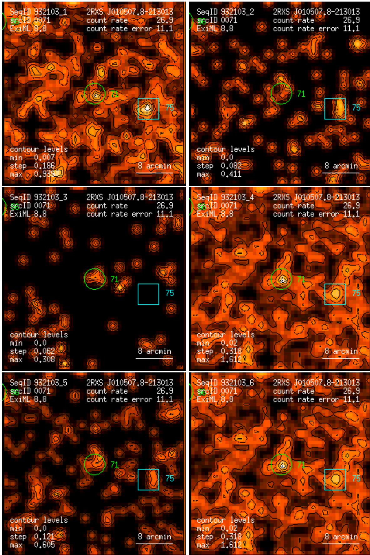
Figure 71: RASS 932103: detection 0071: band rate images, Gaussian filter: (1) PSPC channels 11 – 41, (2) 52 – 90, (3) 91 – 201, (4) 11 – 235, (5) 52 – 201, (6) 11 – 201. Broad band rates in counts/ks. Band rate contour levels in counts/ks/arcmin 2 .
