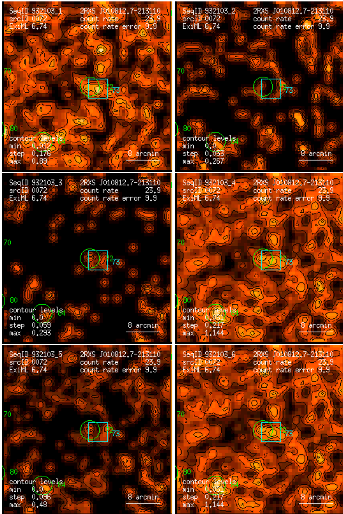
Figure 72: RASS 932103: detection 0072: band rate images, Gaussian filter: (1) PSPC channels 11 – 41, (2) 52 – 90, (3) 91 – 201, (4) 11 – 235, (5) 52 – 201, (6) 11 – 201. Broad band rates in counts/ks. Band rate contour levels in counts/ks/arcmin 2 .
