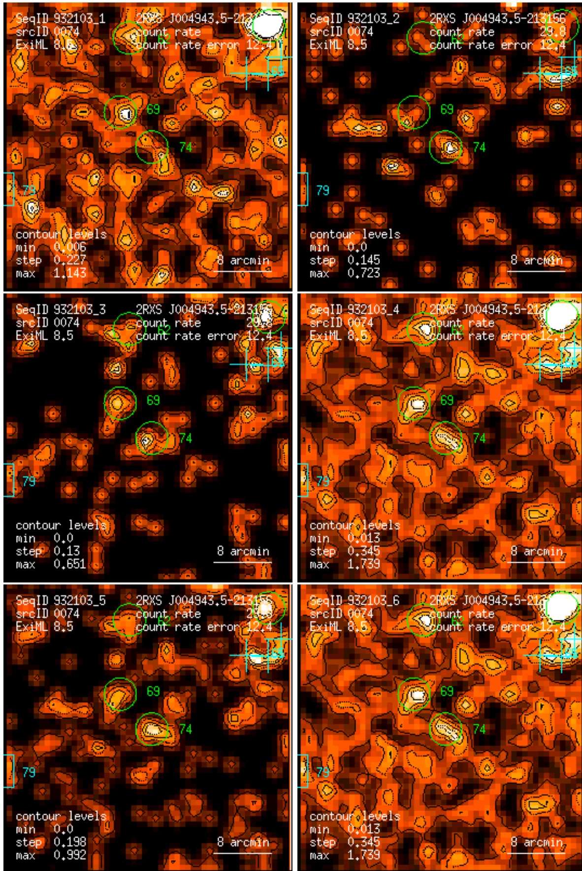
Figure 74: RASS 932103: detection 0074: band rate images, Gaussian filter: (1) PSPC channels 11 – 41, (2) 52 – 90, (3) 91 – 201, (4) 11 – 235, (5) 52 – 201, (6) 11 – 201. Broad band rates in counts/ks. Band rate contour levels in counts/ks/arcmin 2 .
