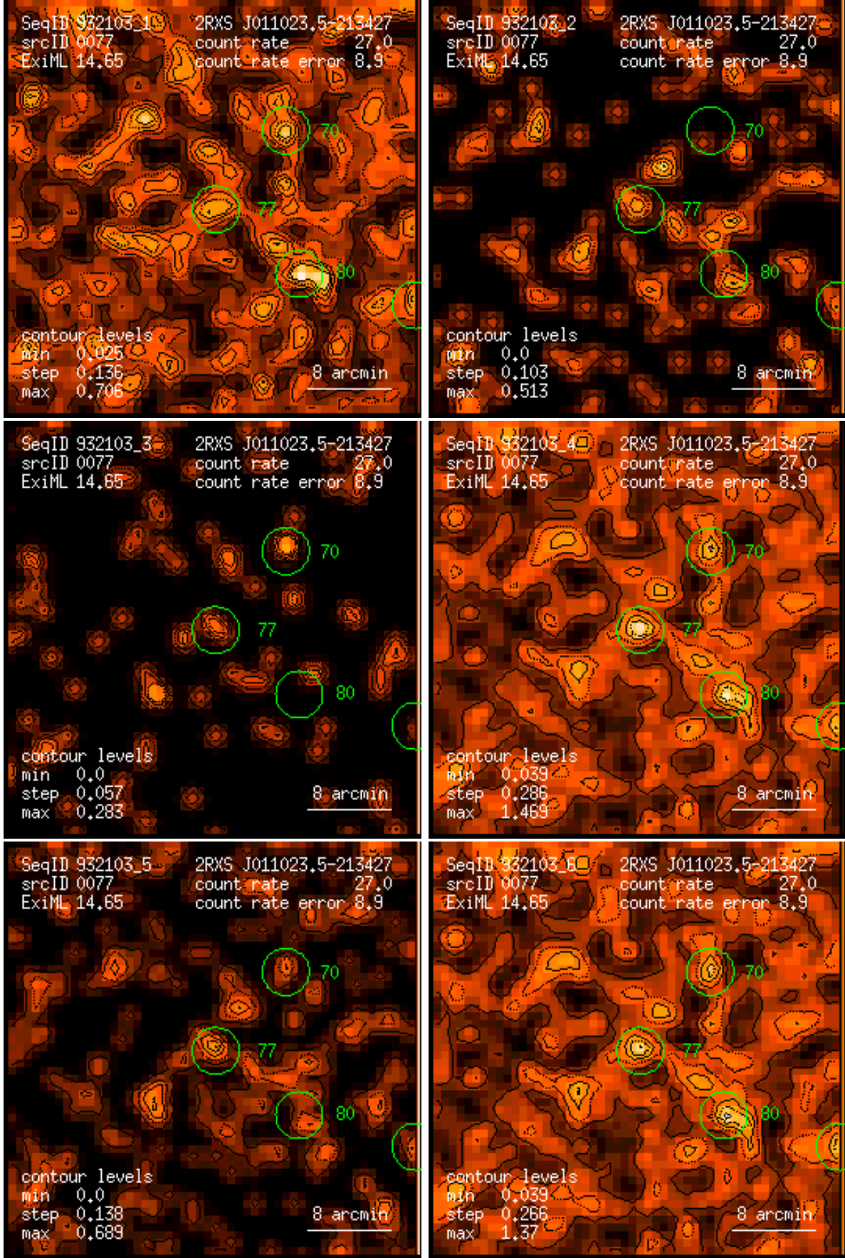
Figure 77: RASS 932103: detection 0077: band rate images, Gaussian filter: (1) PSPC channels 11 – 41, (2) 52 – 90, (3) 91 – 201, (4) 11 – 235, (5) 52 – 201, (6) 11 – 201. Broad band rates in counts/ks. Band rate contour levels in counts/ks/arcmin 2 .
