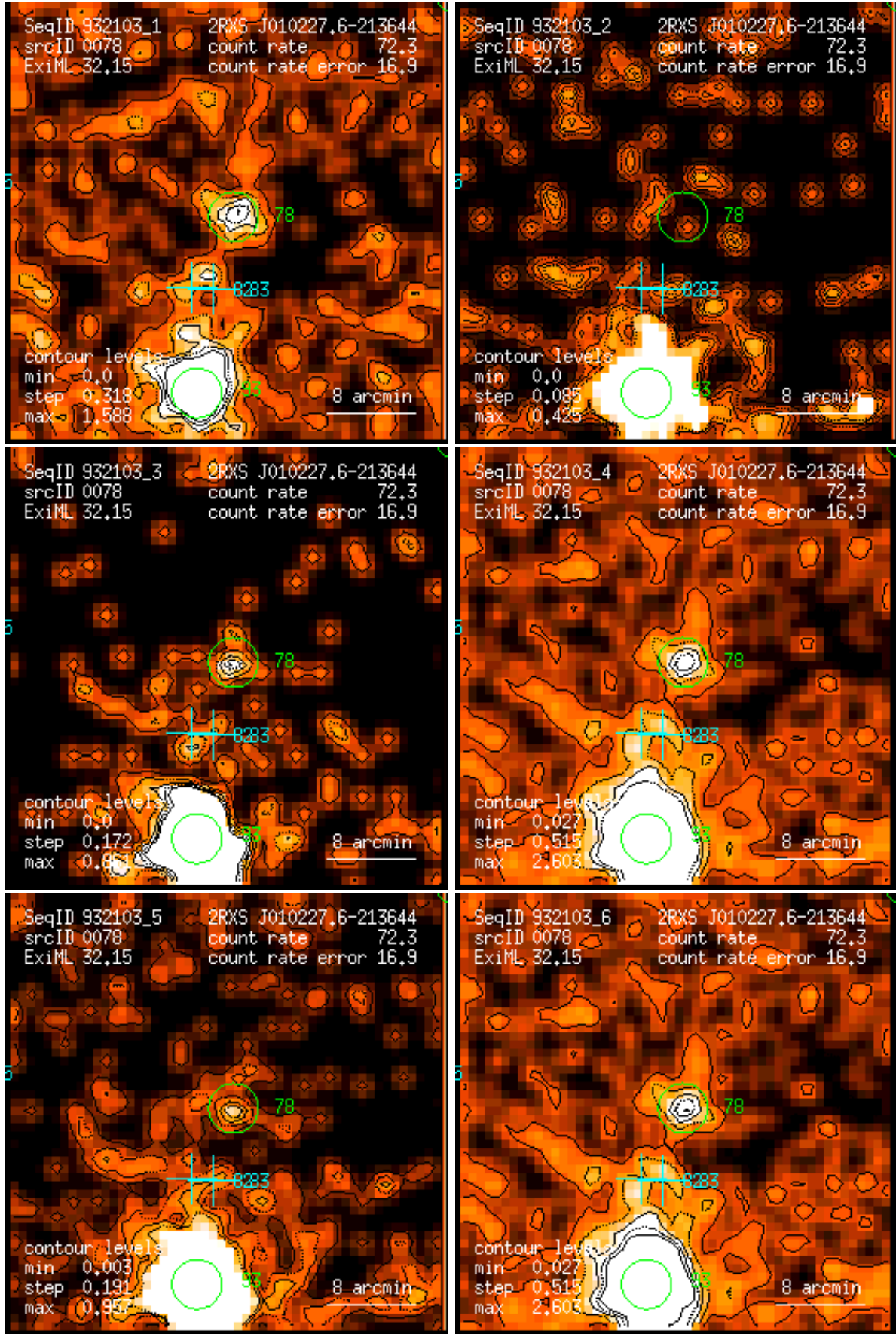
Figure 78: RASS 932103: detection 0078: band rate images, Gaussian filter: (1) PSPC channels 11 – 41, (2) 52 – 90, (3) 91 – 201, (4) 11 – 235, (5) 52 – 201, (6) 11 – 201. Broad band rates in counts/ks. Band rate contour levels in counts/ks/arcmin 2 .
