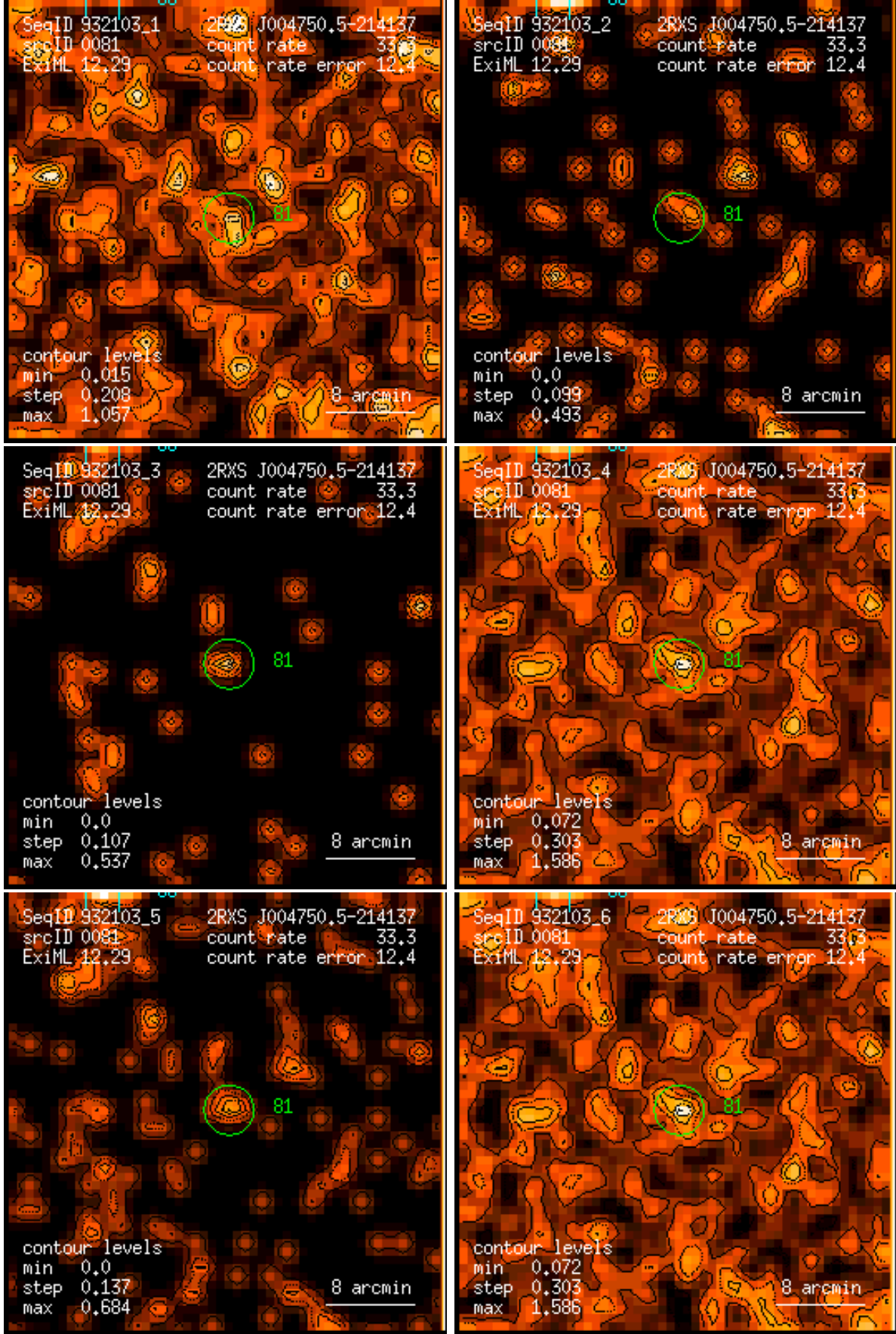
Figure 81: RASS 932103: detection 0081: band rate images, Gaussian filter: (1) PSPC channels 11 – 41, (2) 52 – 90, (3) 91 – 201, (4) 11 – 235, (5) 52 – 201, (6) 11 – 201. Broad band rates in counts/ks. Band rate contour levels in counts/ks/arcmin 2 .
