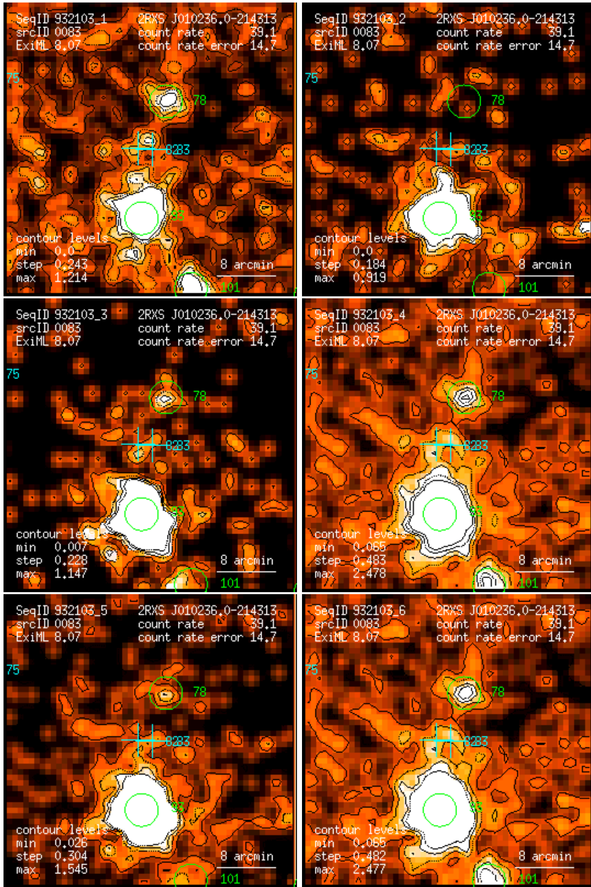
Figure 83: RASS 932103: detection 0083: band rate images, Gaussian filter: (1) PSPC channels 11 – 41, (2) 52 – 90, (3) 91 – 201, (4) 11 – 235, (5) 52 – 201, (6) 11 – 201. Broad band rates in counts/ks. Band rate contour levels in counts/ks/arcmin 2 .
