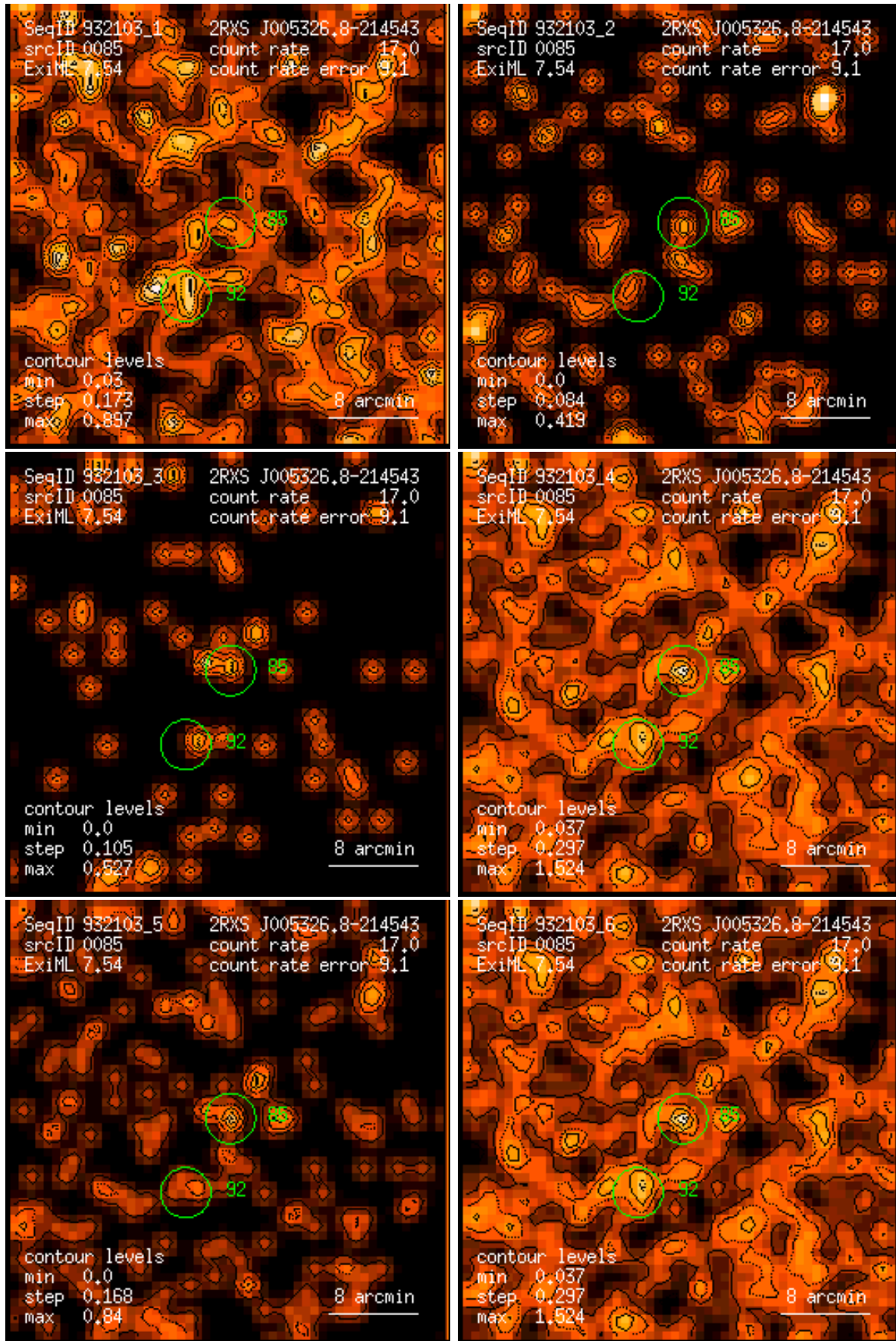
Figure 85: RASS 932103: detection 0085: band rate images, Gaussian filter: (1) PSPC channels 11 – 41, (2) 52 – 90, (3) 91 – 201, (4) 11 – 235, (5) 52 – 201, (6) 11 – 201. Broad band rates in counts/ks. Band rate contour levels in counts/ks/arcmin 2 .
