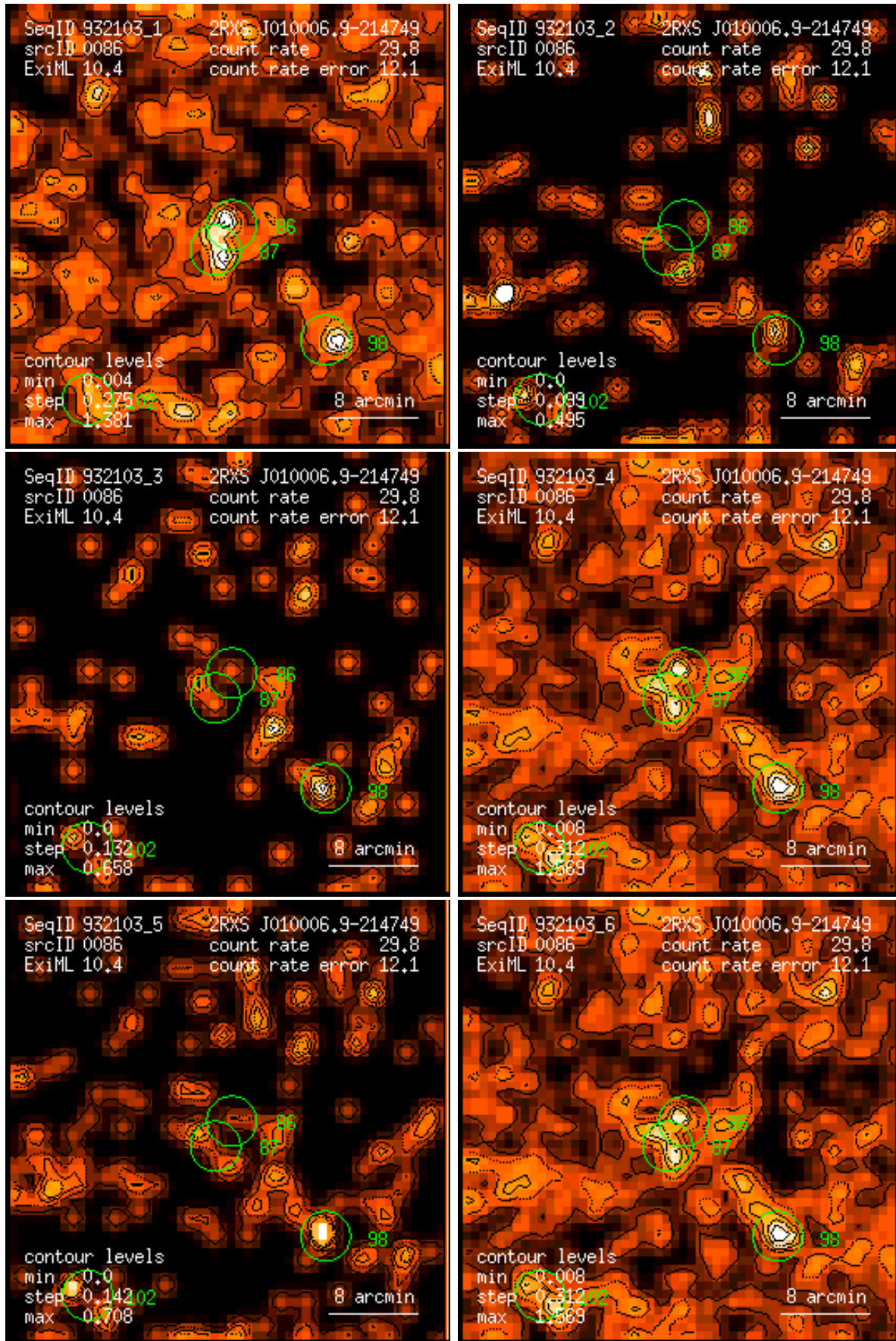
Figure 86: RASS 932103: detection 0086: band rate images, Gaussian filter: (1) PSPC channels 11 – 41, (2) 52 – 90, (3) 91 – 201, (4) 11 – 235, (5) 52 – 201, (6) 11 – 201. Broad band rates in counts/ks. Band rate contour levels in counts/ks/arcmin 2 .
