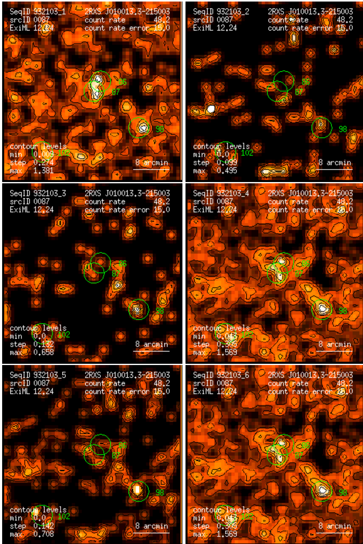
Figure 87: RASS 932103: detection 0087: band rate images, Gaussian filter: (1) PSPC channels 11 – 41, (2) 52 – 90, (3) 91 – 201, (4) 11 – 235, (5) 52 – 201, (6) 11 – 201. Broad band rates in counts/ks. Band rate contour levels in counts/ks/arcmin 2 .
