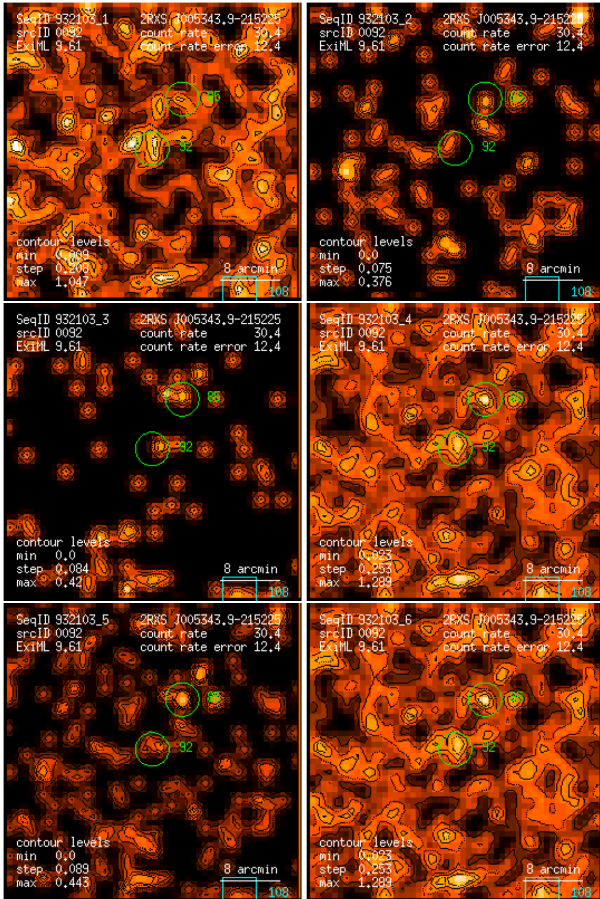
Figure 92: RASS 932103: detection 0092: band rate images, Gaussian filter: (1) PSPC channels 11 – 41, (2) 52 – 90, (3) 91 – 201, (4) 11 – 235, (5) 52 – 201, (6) 11 – 201. Broad band rates in counts/ks. Band rate contour levels in counts/ks/arcmin 2 .
