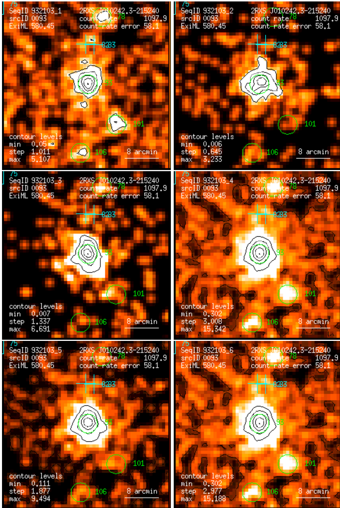
Figure 93: RASS 932103: detection 0093: band rate images, Gaussian filter: (1) PSPC channels 11 – 41, (2) 52 – 90, (3) 91 – 201, (4) 11 – 235, (5) 52 – 201, (6) 11 – 201. Broad band rates in counts/ks. Band rate contour levels in counts/ks/arcmin 2 .
