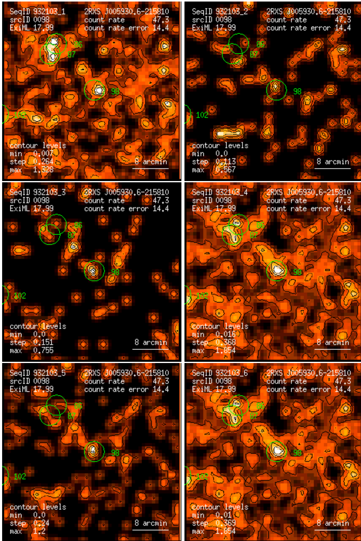
Figure 98: RASS 932103: detection 0098: band rate images, Gaussian filter: (1) PSPC channels 11 – 41, (2) 52 – 90, (3) 91 – 201, (4) 11 – 235, (5) 52 – 201, (6) 11 – 201. Broad band rates in counts/ks. Band rate contour levels in counts/ks/arcmin 2 .
