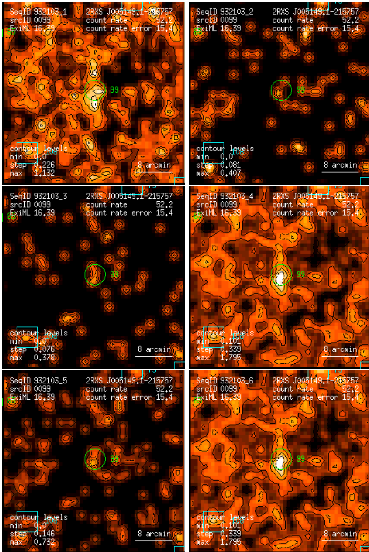
Figure 99: RASS 932103: detection 0099: band rate images, Gaussian filter: (1) PSPC channels 11 – 41, (2) 52 – 90, (3) 91 – 201, (4) 11 – 235, (5) 52 – 201, (6) 11 – 201. Broad band rates in counts/ks. Band rate contour levels in counts/ks/arcmin 2 .
