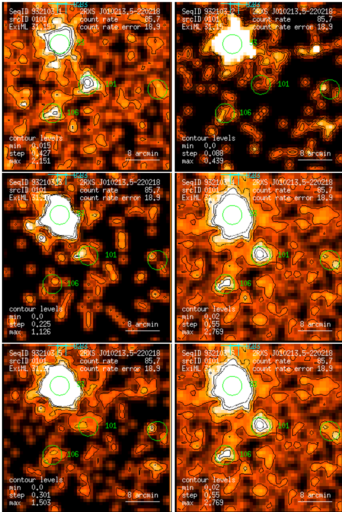
Figure 101: RASS 932103: detection 0101: band rate images, Gaussian filter: (1) PSPC channels 11 – 41, (2) 52 – 90, (3) 91 – 201, (4) 11 – 235, (5) 52 – 201, (6) 11 – 201. Broad band rates in counts/ks. Band rate contour levels in counts/ks/arcmin 2 .
