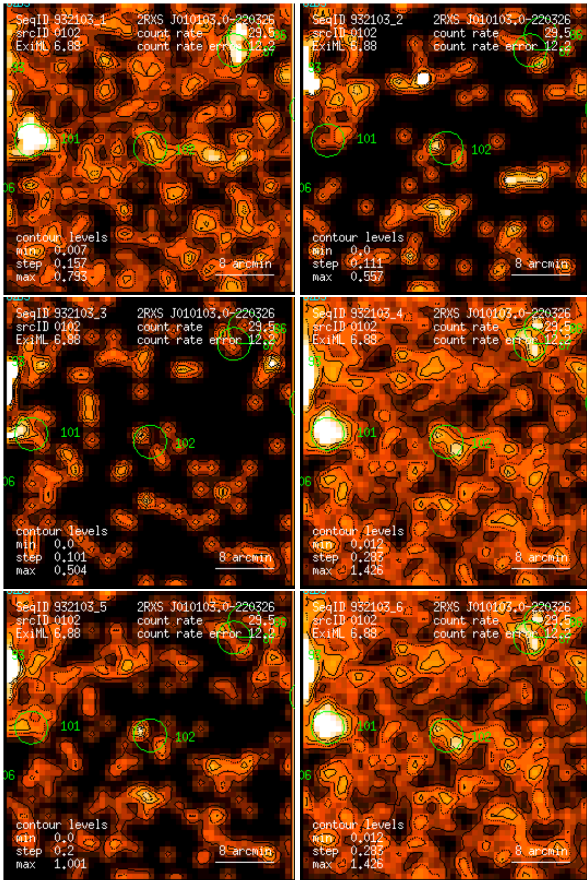
Figure 102: RASS 932103: detection 0102: band rate images, Gaussian filter: (1) PSPC channels 11 – 41, (2) 52 – 90, (3) 91 – 201, (4) 11 – 235, (5) 52 – 201, (6) 11 – 201. Broad band rates in counts/ks. Band rate contour levels in counts/ks/arcmin 2 .
