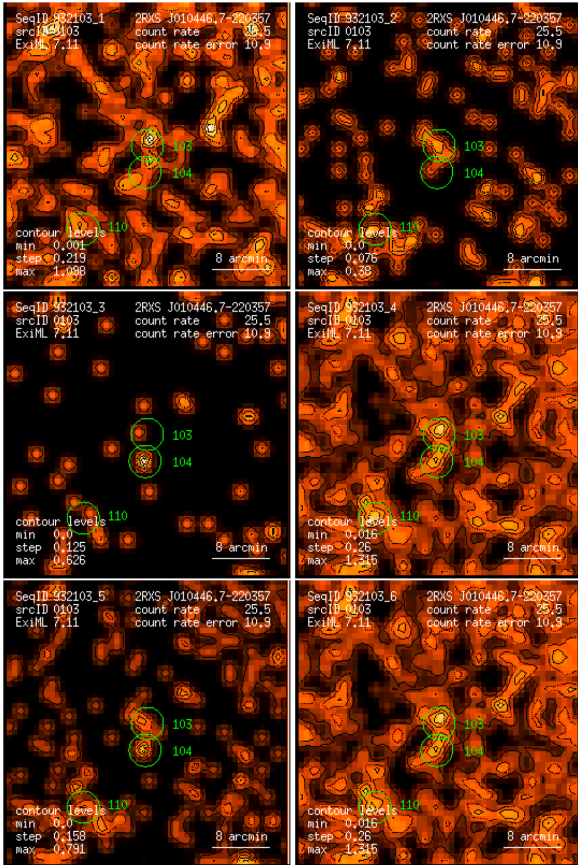
Figure 103: RASS 932103: detection 0103: band rate images, Gaussian filter: (1) PSPC channels 11 – 41, (2) 52 – 90, (3) 91 – 201, (4) 11 – 235, (5) 52 – 201, (6) 11 – 201. Broad band rates in counts/ks. Band rate contour levels in counts/ks/arcmin 2 .
