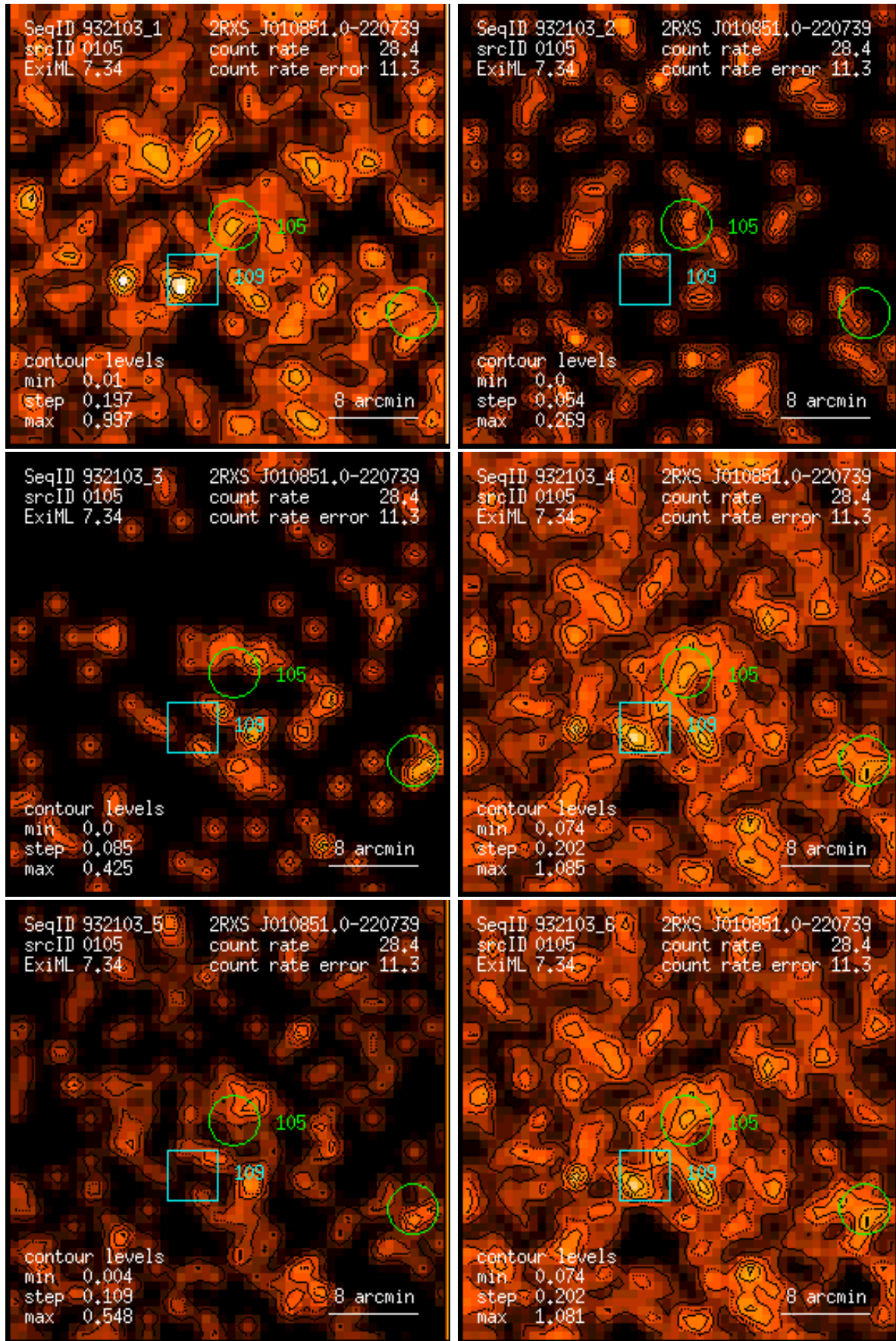
Figure 105: RASS 932103: detection 0105: band rate images, Gaussian filter: (1) PSPC channels 11 – 41, (2) 52 – 90, (3) 91 – 201, (4) 11 – 235, (5) 52 – 201, (6) 11 – 201. Broad band rates in counts/ks. Band rate contour levels in counts/ks/arcmin 2 .
