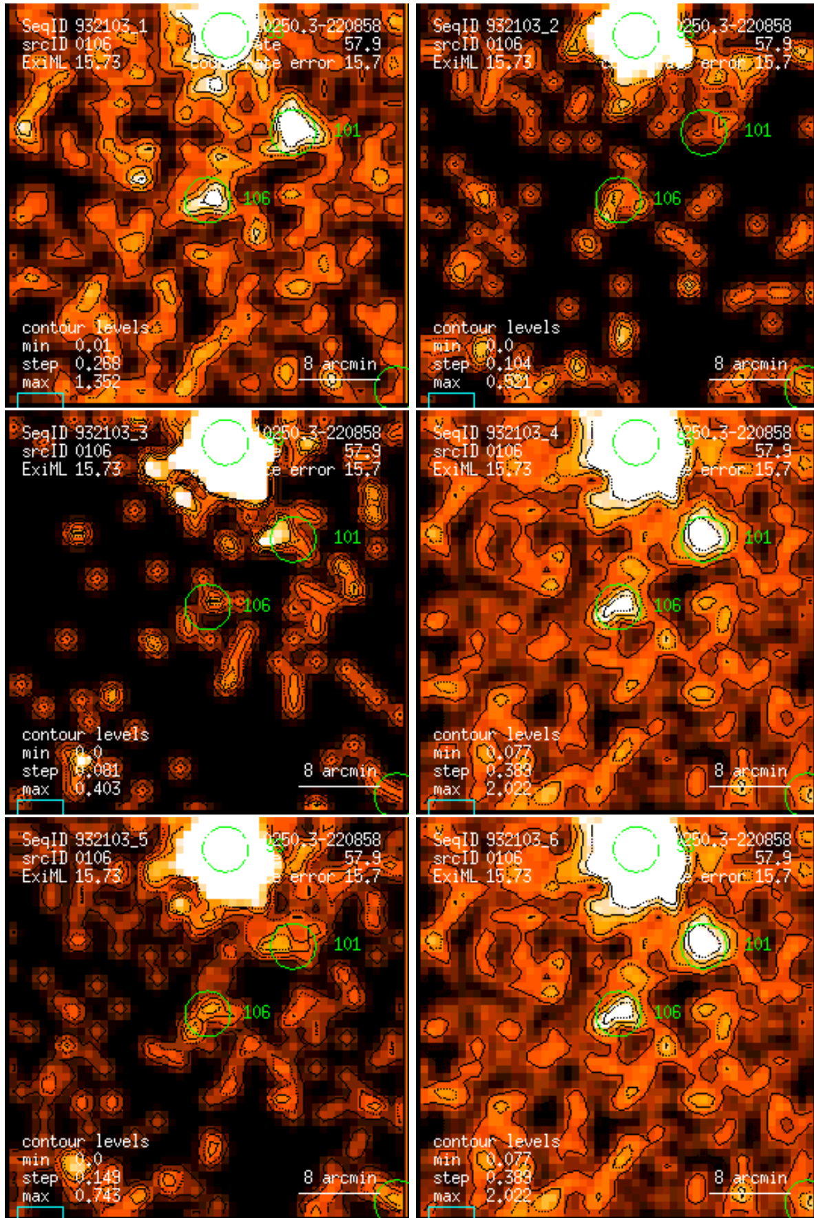
Figure 106: RASS 932103: detection 0106: band rate images, Gaussian filter: (1) PSPC channels 11 – 41, (2) 52 – 90, (3) 91 – 201, (4) 11 – 235, (5) 52 – 201, (6) 11 – 201. Broad band rates in counts/ks. Band rate contour levels in counts/ks/arcmin 2 .
