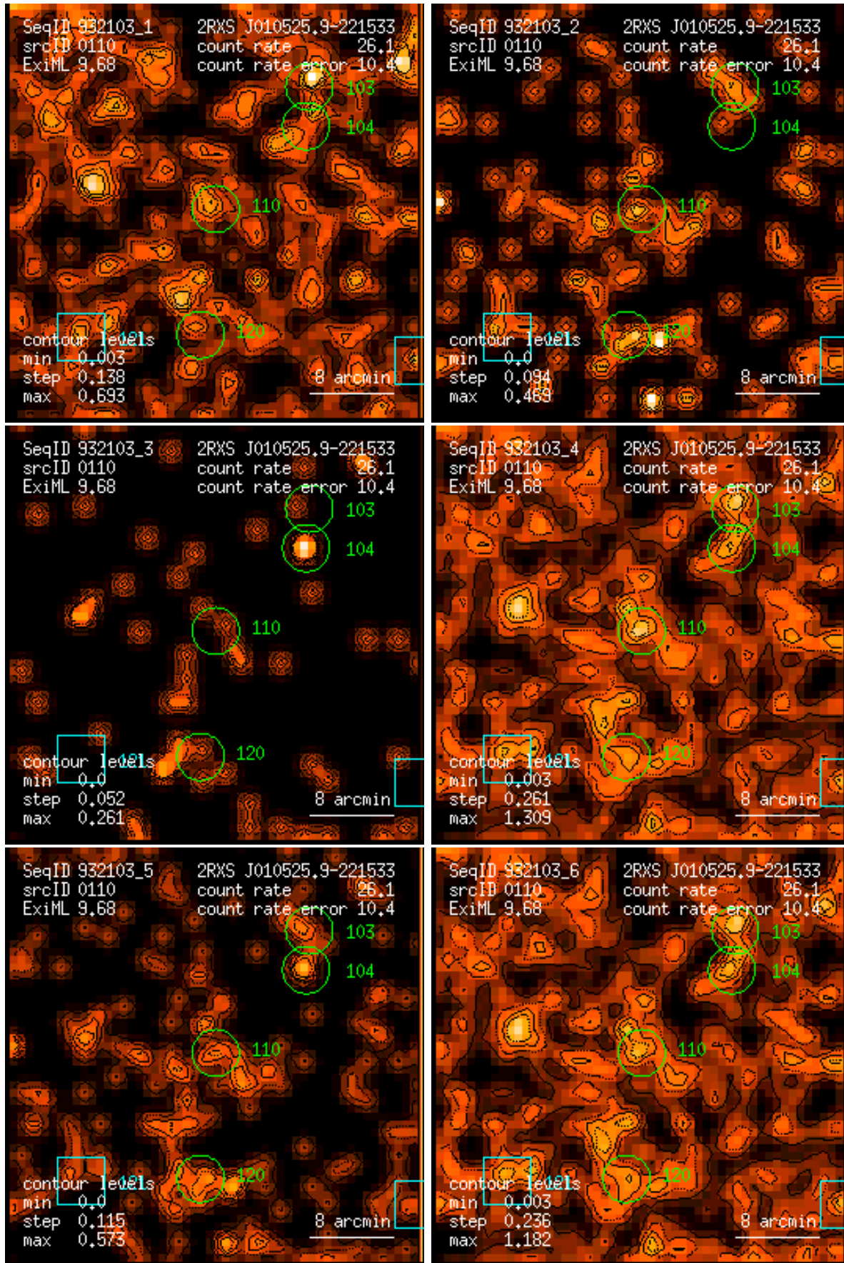
Figure 110: RASS 932103: detection 0110: band rate images, Gaussian filter: (1) PSPC channels 11 – 41, (2) 52 – 90, (3) 91 – 201, (4) 11 – 235, (5) 52 – 201, (6) 11 – 201. Broad band rates in counts/ks. Band rate contour levels in counts/ks/arcmin 2 .
