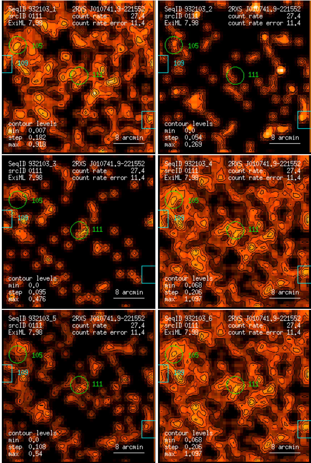
Figure 111: RASS 932103: detection 0111: band rate images, Gaussian filter: (1) PSPC channels 11 – 41, (2) 52 – 90, (3) 91 – 201, (4) 11 – 235, (5) 52 – 201, (6) 11 – 201. Broad band rates in counts/ks. Band rate contour levels in counts/ks/arcmin 2 .
