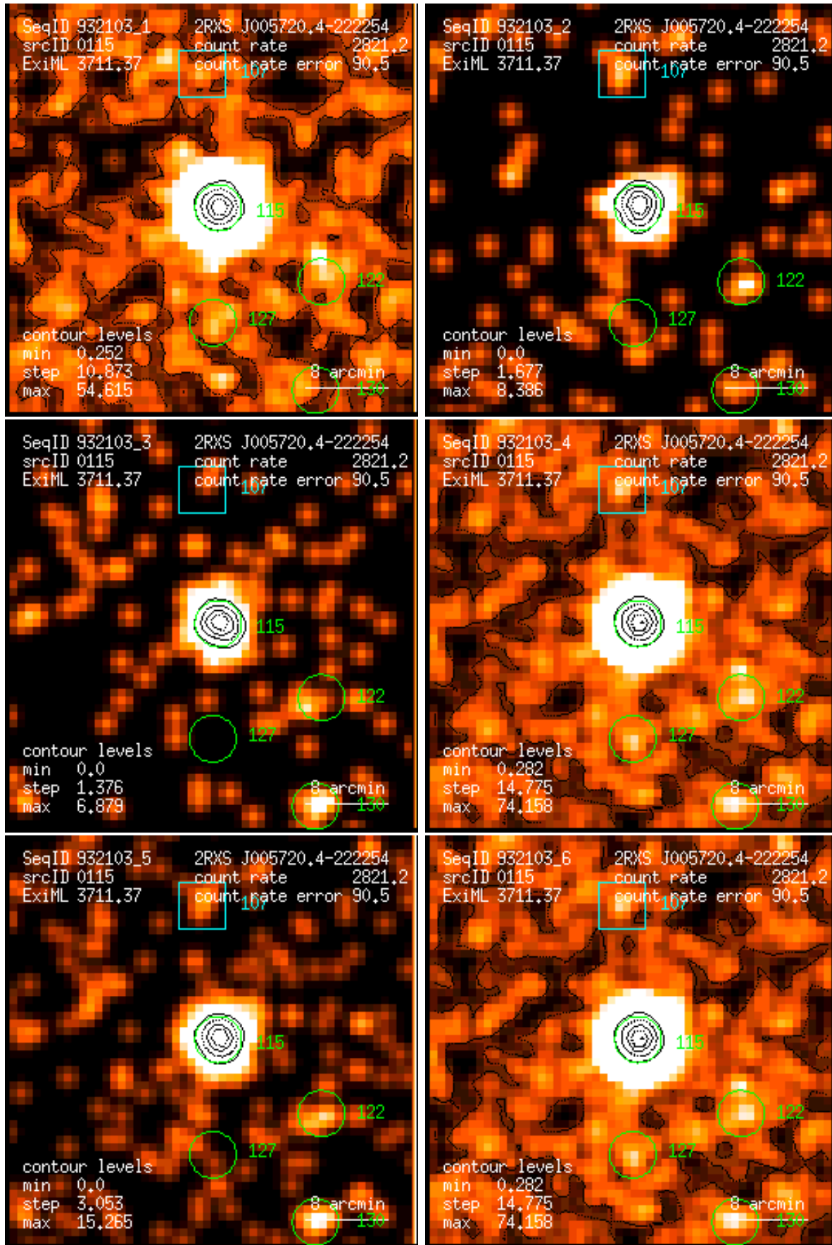
Figure 115: RASS 932103: detection 0115: band rate images, Gaussian filter: (1) PSPC channels 11 – 41, (2) 52 – 90, (3) 91 – 201, (4) 11 – 235, (5) 52 – 201, (6) 11 – 201. Broad band rates in counts/ks. Band rate contour levels in counts/ks/arcmin 2 .
