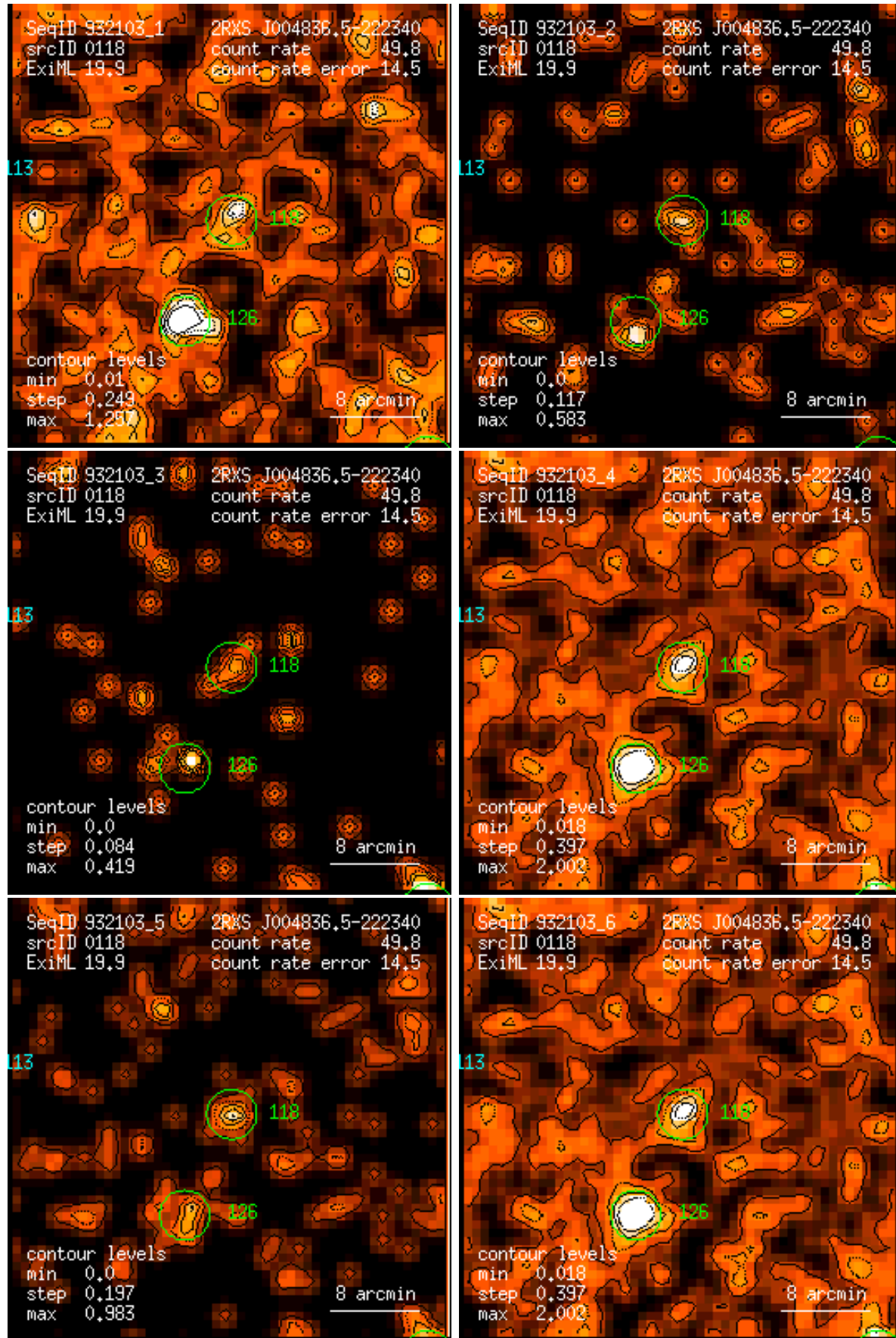
Figure 118: RASS 932103: detection 0118: band rate images, Gaussian filter: (1) PSPC channels 11 – 41, (2) 52 – 90, (3) 91 – 201, (4) 11 – 235, (5) 52 – 201, (6) 11 – 201. Broad band rates in counts/ks. Band rate contour levels in counts/ks/arcmin 2 .
