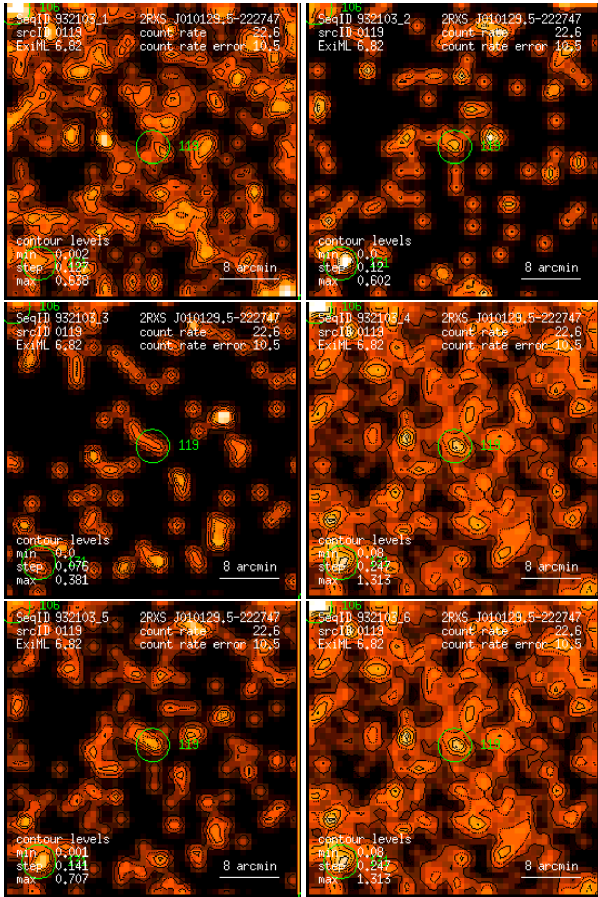
Figure 119: RASS 932103: detection 0119: band rate images, Gaussian filter: (1) PSPC channels 11 – 41, (2) 52 – 90, (3) 91 – 201, (4) 11 – 235, (5) 52 – 201, (6) 11 – 201. Broad band rates in counts/ks. Band rate contour levels in counts/ks/arcmin 2 .
