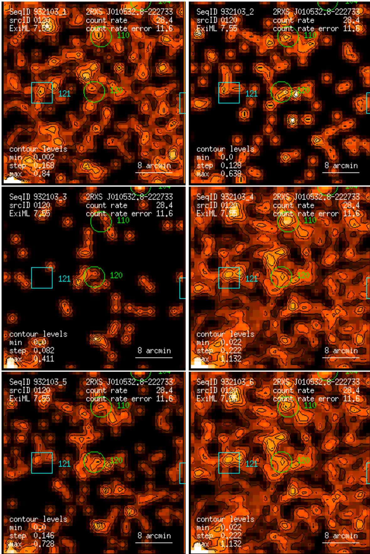
Figure 120: RASS 932103: detection 0120: band rate images, Gaussian filter: (1) PSPC channels 11 – 41, (2) 52 – 90, (3) 91 – 201, (4) 11 – 235, (5) 52 – 201, (6) 11 – 201. Broad band rates in counts/ks. Band rate contour levels in counts/ks/arcmin 2 .
